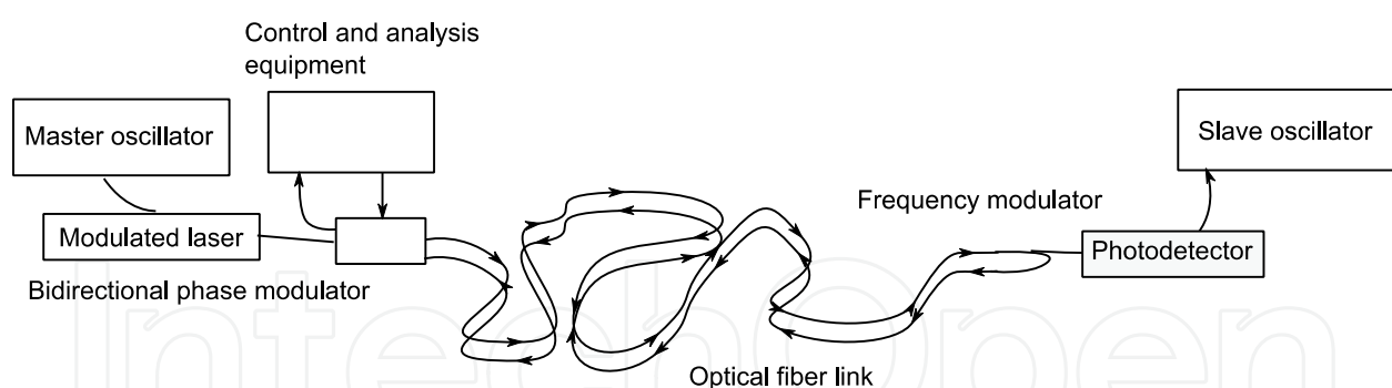
Fig. 9. Schematic frequency transfer in microwave domain.
