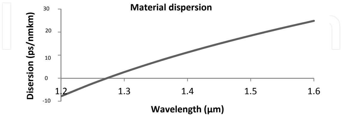
Fig. 5. Calculation of material dispersion in Fused Silica at 20°C.
