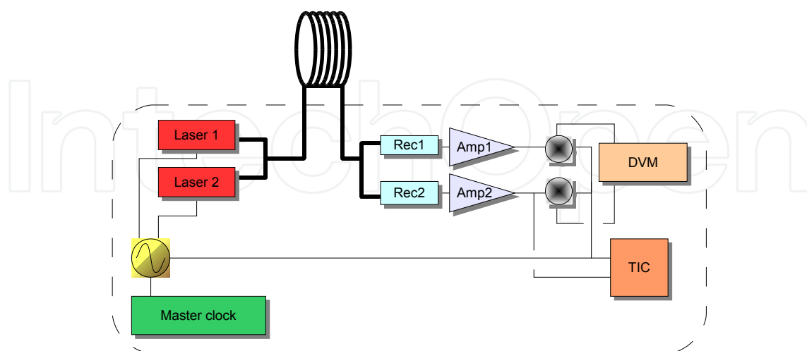
Fig. 7. Experimental setup. Rec1 and Rec2 include optical pre-amplification, optical band pass filter, photodiode and electrical trans-impedance amplifier. Amp1 and Amp2 are electrical amplifiers, DVM digital voltmeter and TIC is time-interval counter. Thin lines symbolize electrical wires and thick lines optical fibers.
