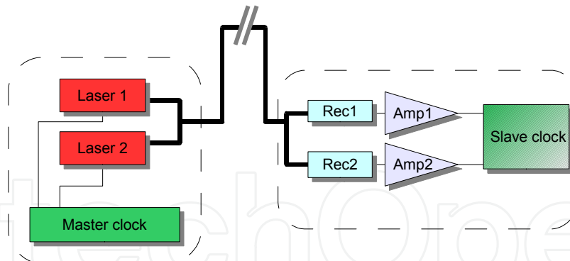
Fig. 4. Schematic system for one-way fiber based time transfer.
