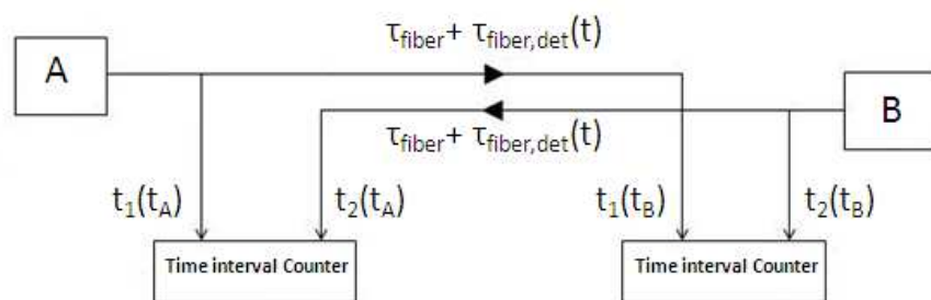
Fig. 3. Schematic system for two-way time transfer.
