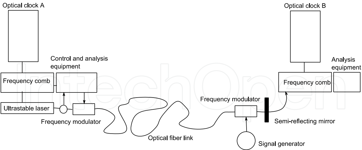
Fig. 11. Schematic setup for optical frequency transfer.
