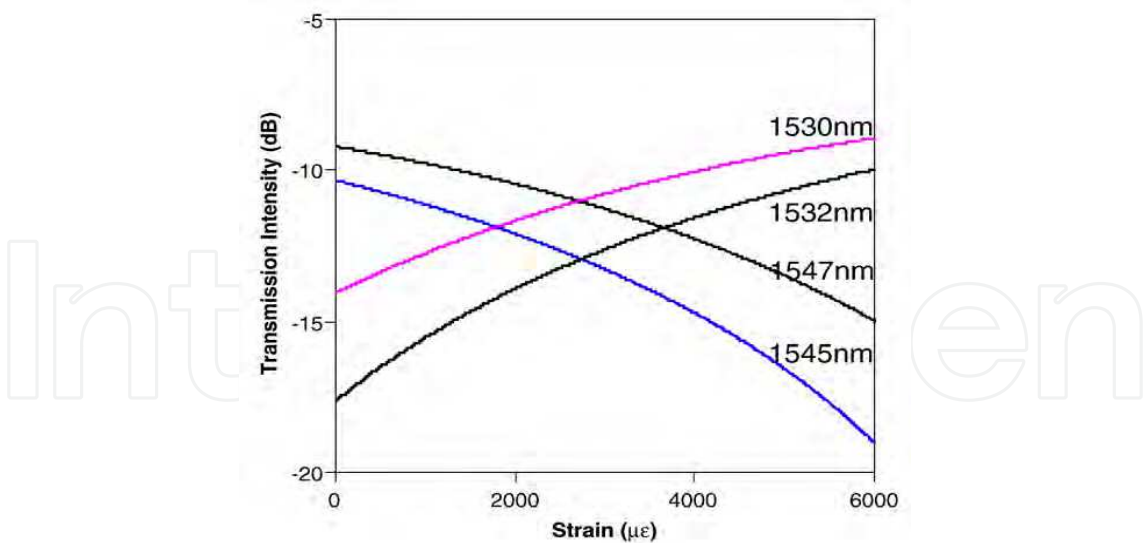
Fig. 26. Theoretical strain dependence of the transmission intensity of the FLM at different wavelengths in the strain range of 0~6000 με.
