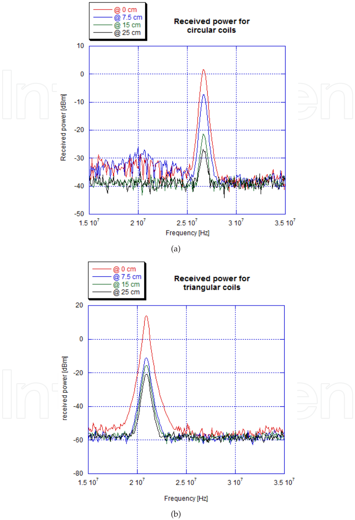
Fig. 8. Received power for different distances. (a) Circular and (b) triangular coils.
