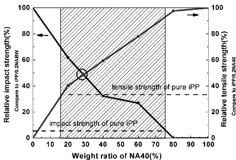
Fig. 8. Effect of NA40/NABW compounded NAs with different ratio on mechanical properties of iPP (addition amount 0.2wt %) (Shi & Xin, 2011)
