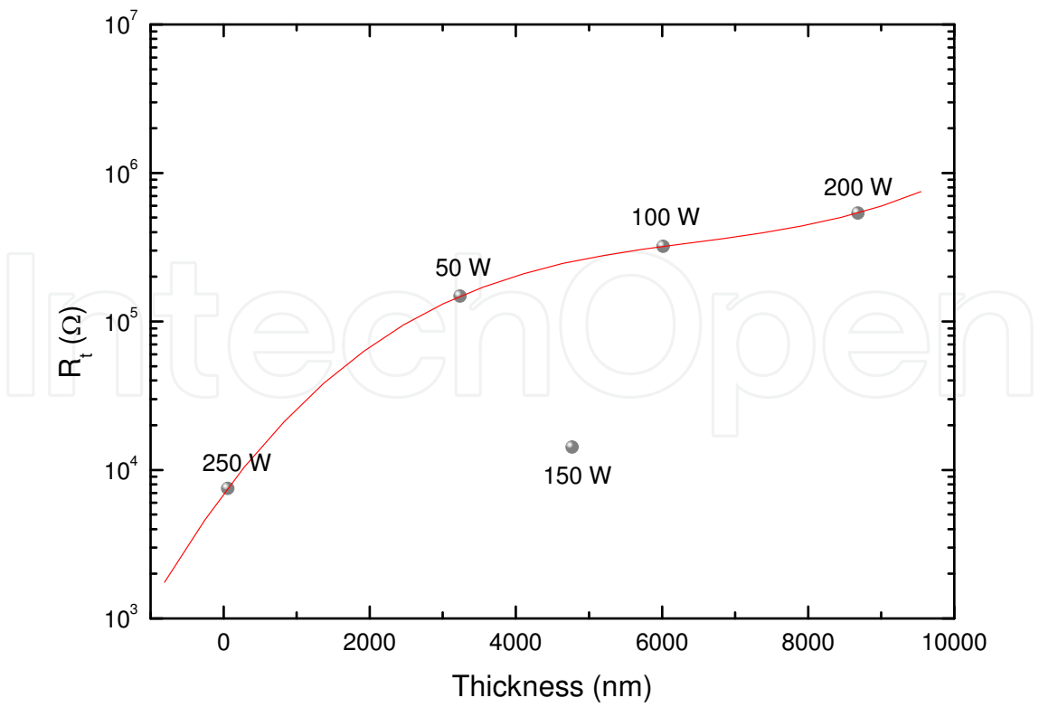
Fig. 14. Total resistance at t = 180 minutes as a function of the film thickness.
