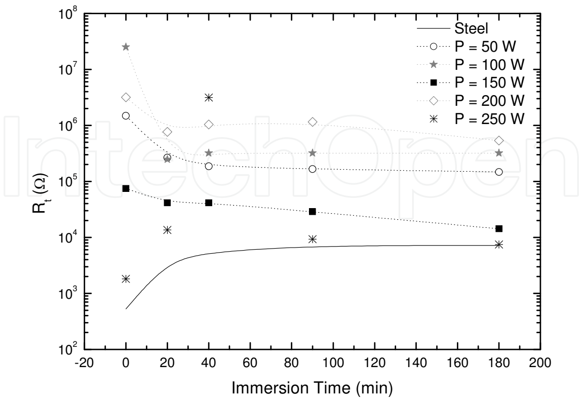
Fig. 13. Total resistance as a function of the immersion time for the samples exposed to plasmas of different powers and for the bare substrate.
