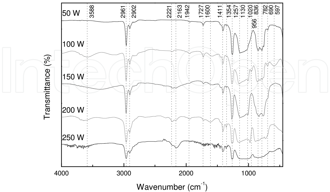
Fig. 4. Infrared spectra of films deposited in plasmas of different powers.
