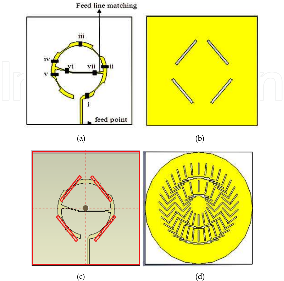
Fig. 1. Simulation structure of the proposed antenna (a) feed line (b) Aperture slots (c) Alignment of aperture slots and feed line (d) RLSA radiating surface
