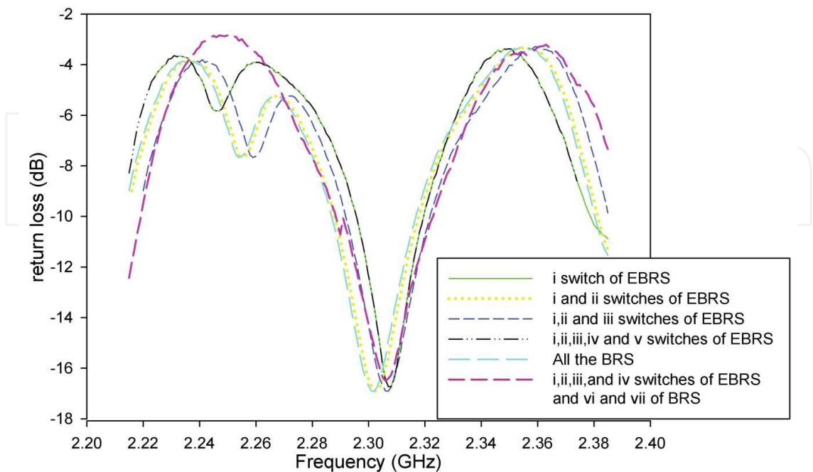
Fig. 9. The measurement of return loss by variation activation of the EBRS and BRS
