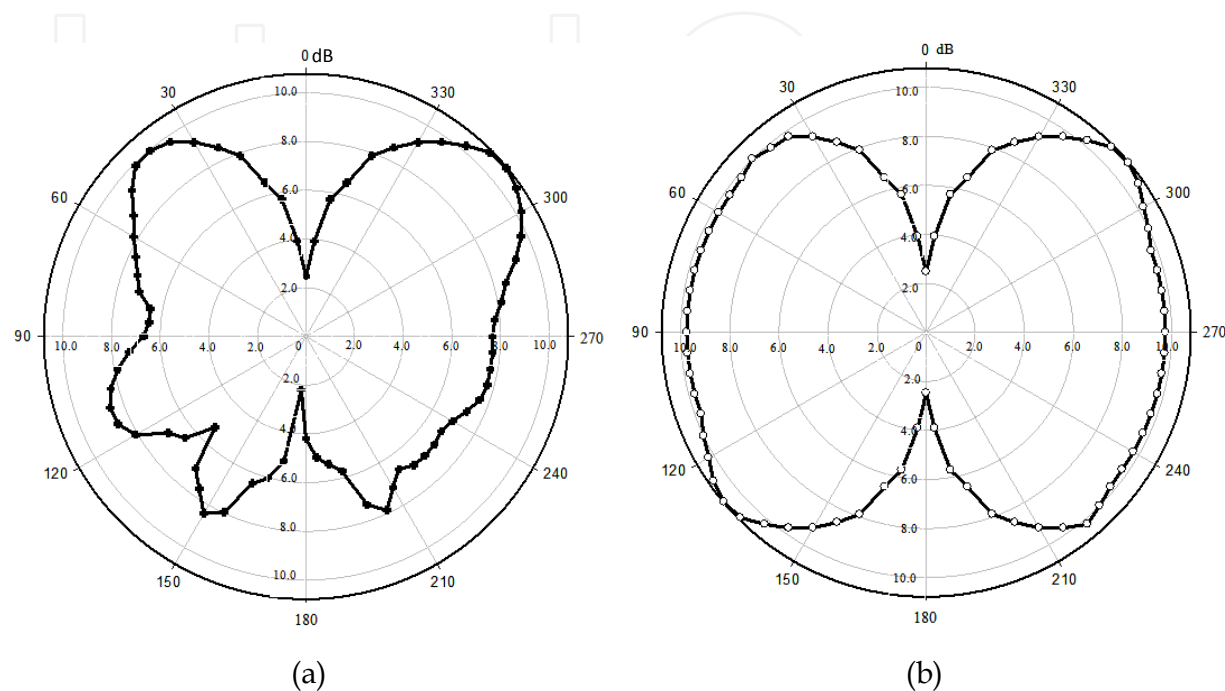
Fig. 6. Broadside divisive radiation patterns (a) Measured (b) Simulation
