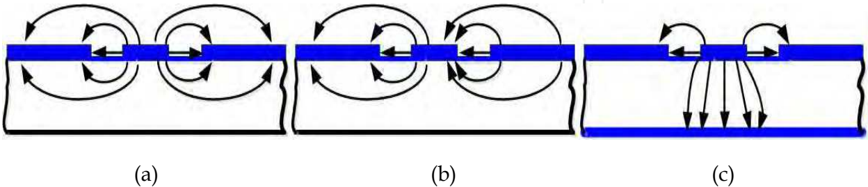
Fig. 2. Schematic electrical field distribution in coplanar waveguide: (a) desired even mode, (b) parasitic odd mode, and (c) parasitic parallel plate mode
