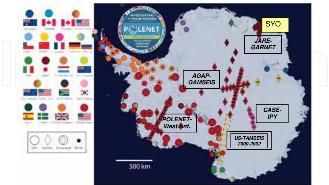
Fig. 15. Distribution map of seismic and the other geophysical stations deployed during the IPY 2007-2008. The major project names are labeled as; JARE-GARNET, AGAP-GAMSEIS, CASE-IPY, POLENET-West.Ant. and US-TAMSEIS, respectively. All stations in Antarctic continent contributed to POLENET program
