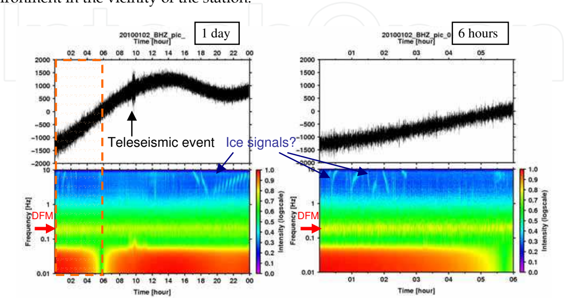
Fig. 3. The power spectral densities (PSD) of the vertical broadband seismometer (STS-1V) at SYO for January 02, 2010. Left: one day of data. Right: 6 hours of data, corresponding to the shadowed area of the left figure.
