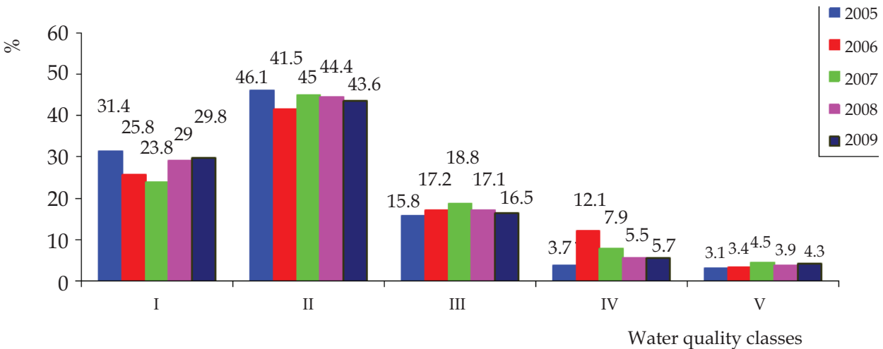
Fig. 6. The surface water distribution by 5 qualities, and by years, during the period of five years 2005 - 2009
