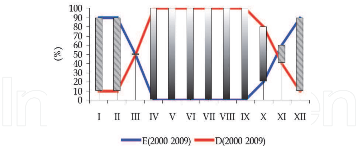
Fig. 13. Percent interannual variations of deficits D and surpluses E of precipitation to potential evapotranspiration for the period 2000 - 2009.
