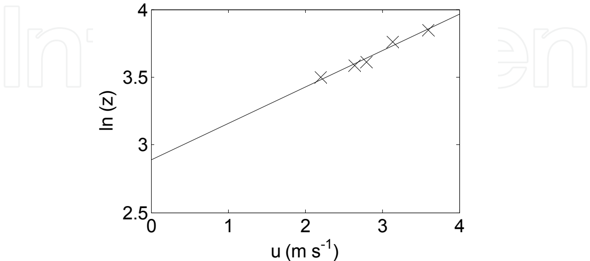
Fig. 2. Example plot of mean wind speed u against \ln(z) , measured above a 31 m tall forest in The Netherlands in August 2009. The intercept with the vertical axis leads to z_{0m}+d = 17.9 m.
