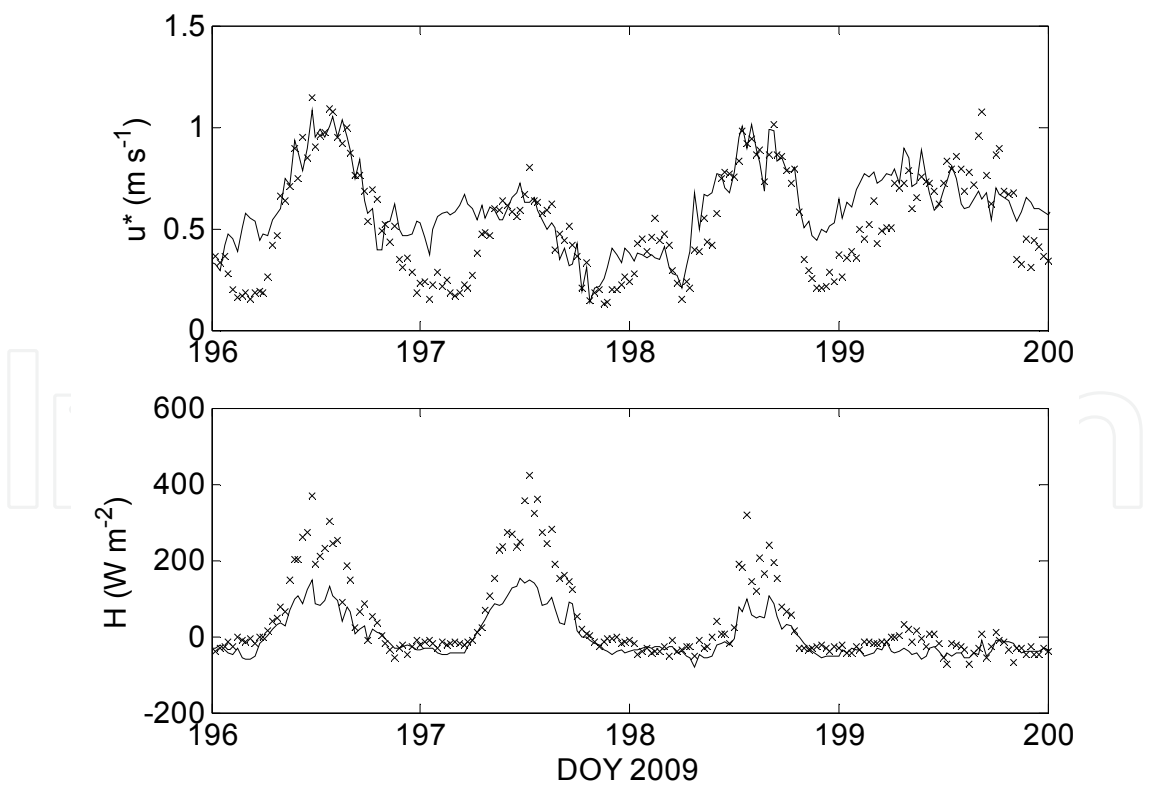
Fig. 5. Measured (symbols) and modeled (line) friction velocity u^* and sensible heat H flux versus Julian day number (14-19 July 2009) for an eddy covariance tower in the Speulderbos forest site, The Netherlands.
