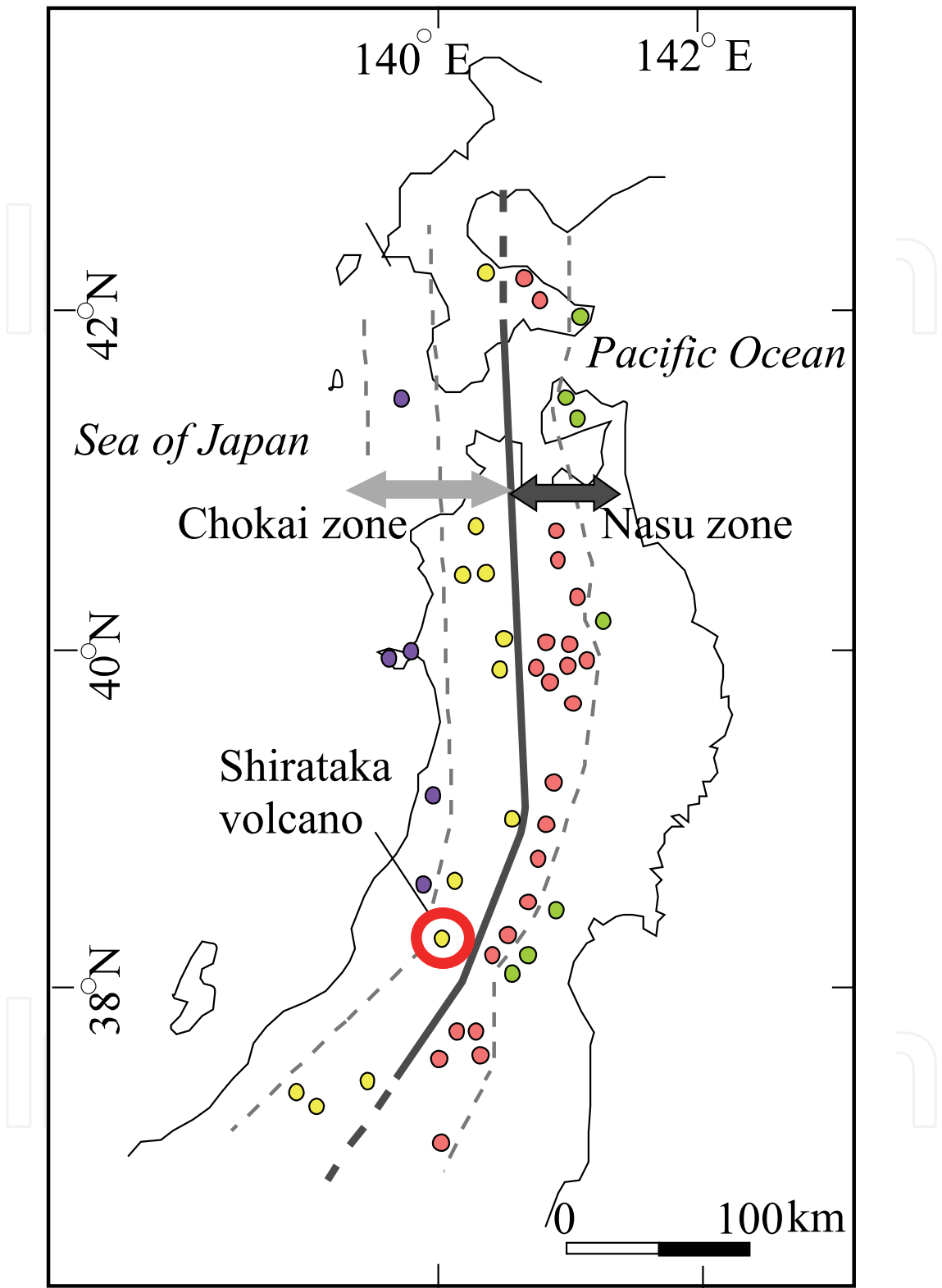
Fig. 1. Location of the Shirataka volcano in the northeast Japan arc. Circles represent Quaternary stratovolcanoes in the northeast Japan arc. The distribution of the volcanoes is from Nakagawa et al. (1988). The distribution of the volcanoes are divided into four volcanic zones: Aoso-Osore (green circle), Sekiryō (orange circle), Moriyoshi (yellow circle), and Chokai (purple circle) zones from trench to rear arc side (Nakagawa et al., 1988).
