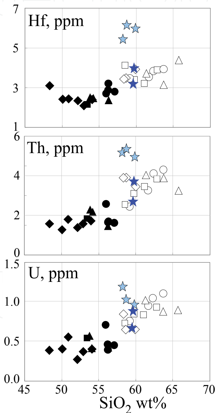
Fig. 4. Hf, Th, and U contents against SiO 2 contents of the samples from the Shirataka volcano. Symbols are the same as in Fig. 2.
