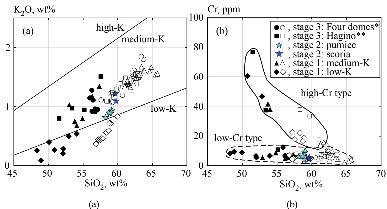
Fig. 2. K_2O vs. SiO_2 (a), in the left figure Cr vs. SiO_2 (b) in the right figure variation diagrams of the eruptive products from the Shirataka volcano (modified after Hirotsu et al., 2009). Data are from Hirotsu & Ban (2006). The boundary lines between low-K and medium-K, and medium-K and high-K are from Gill (1981). Filled symbols are mafic inclusions and open ones are host rocks. *Four domes consist of the Shiratakayama, Kitsunegoe, Nishikuromoriyama lava dome group + Higashikuromoriyama lava dome; **Hagino, the Hagino block-and-ash flow deposit
