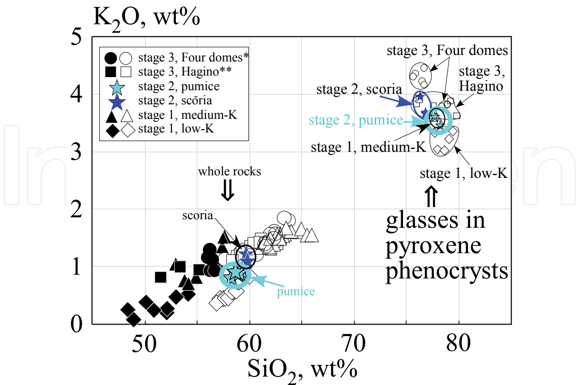
Fig. 5. K_2O - SiO_2 diagram showing the compositions of glass inclusions in pyroxene phenocrysts from each stage in the Shirataka volcano. *Four domes, the Shiratakayama, Kitsunegoe, Nishikuromoriyama lava dome group + Higashikuromoriyama lava dome; **Hagino, the Hagino block-and-ash flow deposit
