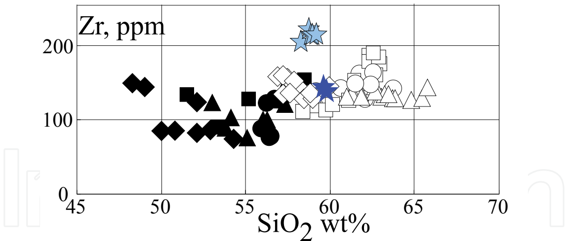
Fig. 3. Zr vs. SiO 2 diagram of the eruptive products from the Shirataka volcano (modified after Hirotsu & Ban, 2006). Data are from Hirotsu & Ban (2006). Symbols are the same as in Fig. 2.
