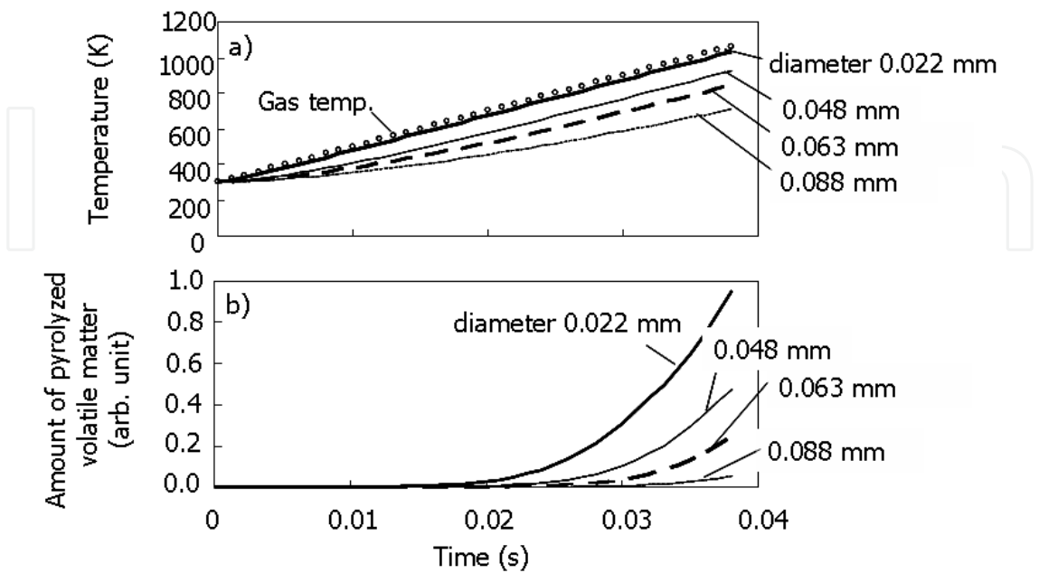
Fig. 12. Effect of particle diameter on pyrolysis property.
