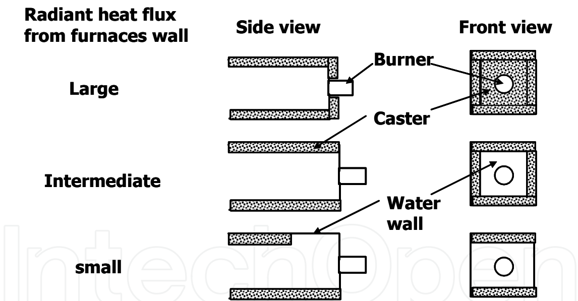
Fig. 24. Example of procedure to evaluate the effect of the radiant heat flux for large scale burners [36].
