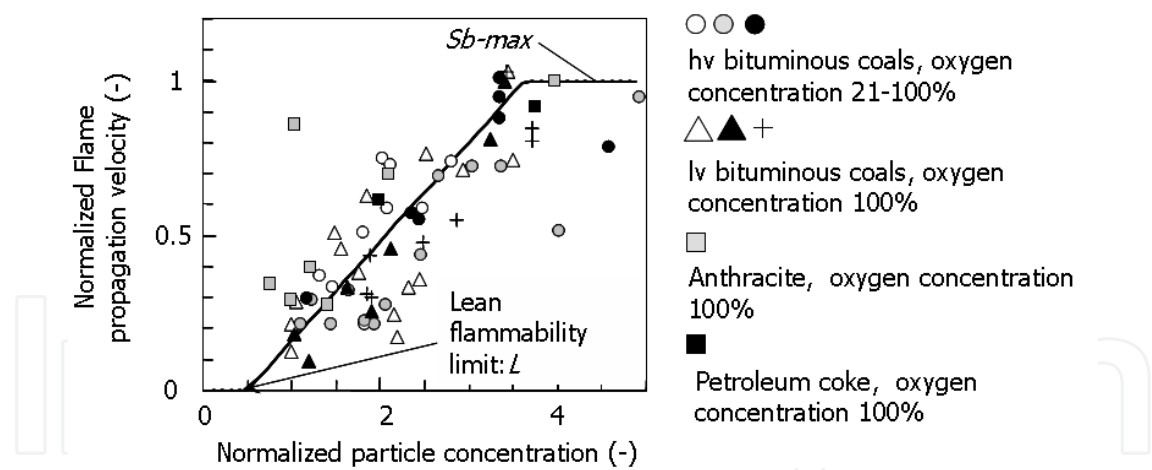
Fig. 7. Relationship between coal concentration and flame propagation velocity [12].
