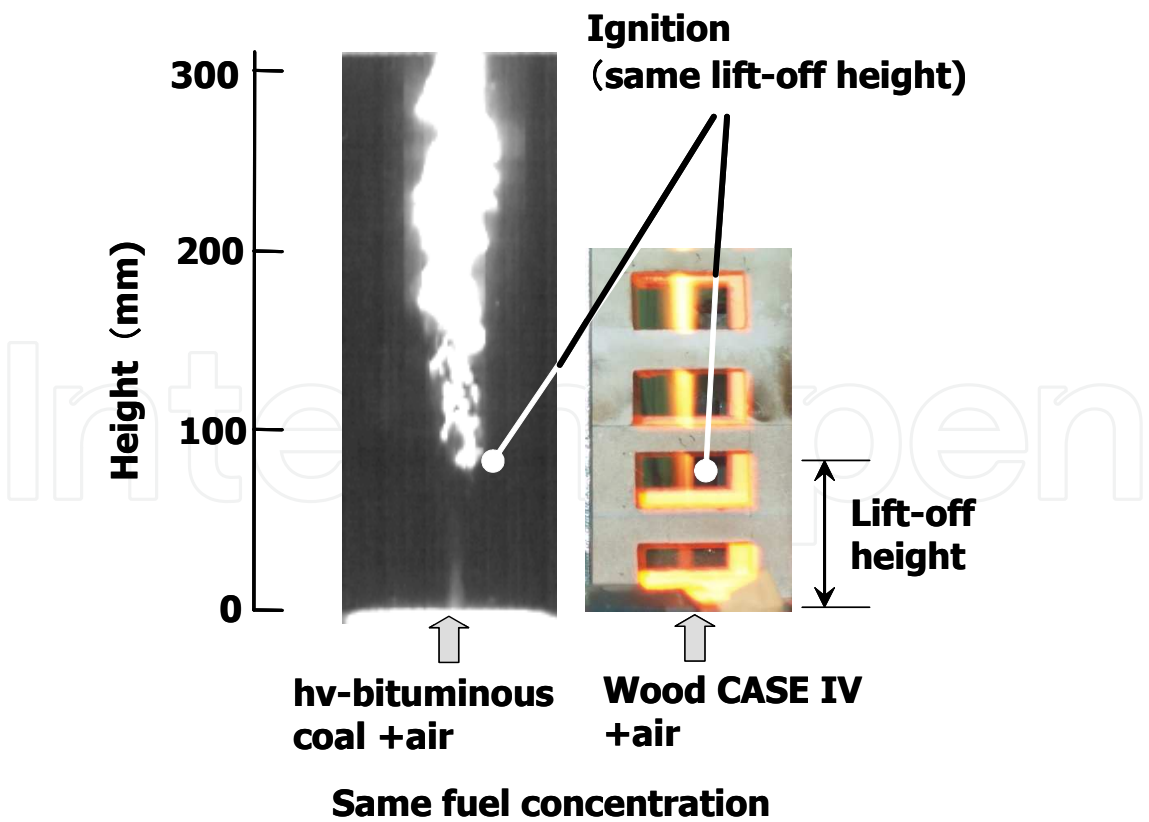
Fig. 27. Comparison of lift-off heights between hv-bituminous coal and wood powder for the same primary fuel concentrations.
