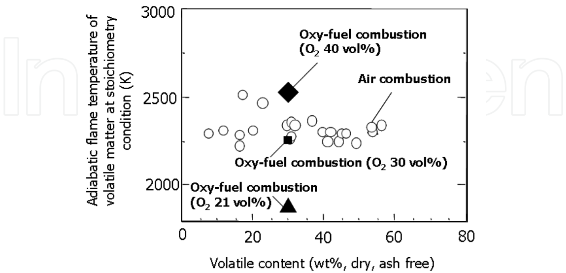
Fig. 15. Calculated adiabatic flame temperatures of volatile matter at stoichiometry condition, under various coals and surrounding gas compositions.
