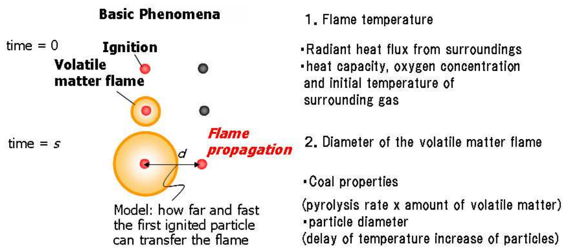
Fig. 6. Basic model for flame propagation.
