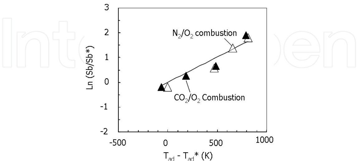
Fig. 14. Relationship between flame propagation velocity and flame temperature formed around the particle [12]. Experimental data were obtained from Suda et al. [9].
