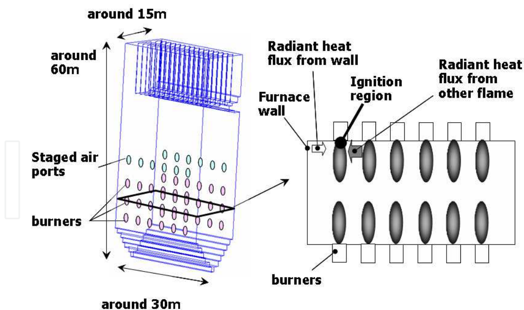
Fig. 22. Example burner arrangement of a pulverized coal fired boiler.
