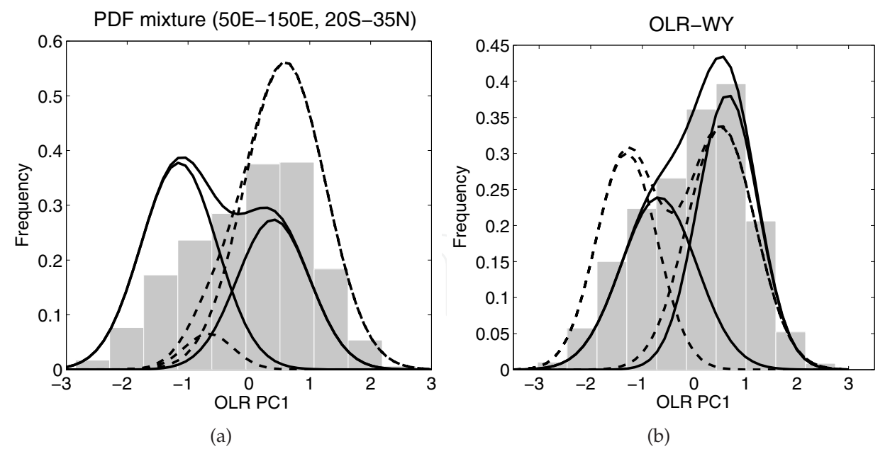
Fig. 10. (a) PDFs of the daily OLR time series in the early (solid) and late (dashed) part of the record. Upper (lower) curves represent total (mixture components) probability distributions. The left (right) component of the mixture represents regime R1 (R2). (b) Perturbations to the whole period mixture when the OLR index is stratified by JJAS-average dynamical monsoon, or Webster-Yang, index: WY^+ (dashed) and WY^- (solid). Reproduced from TH10.
