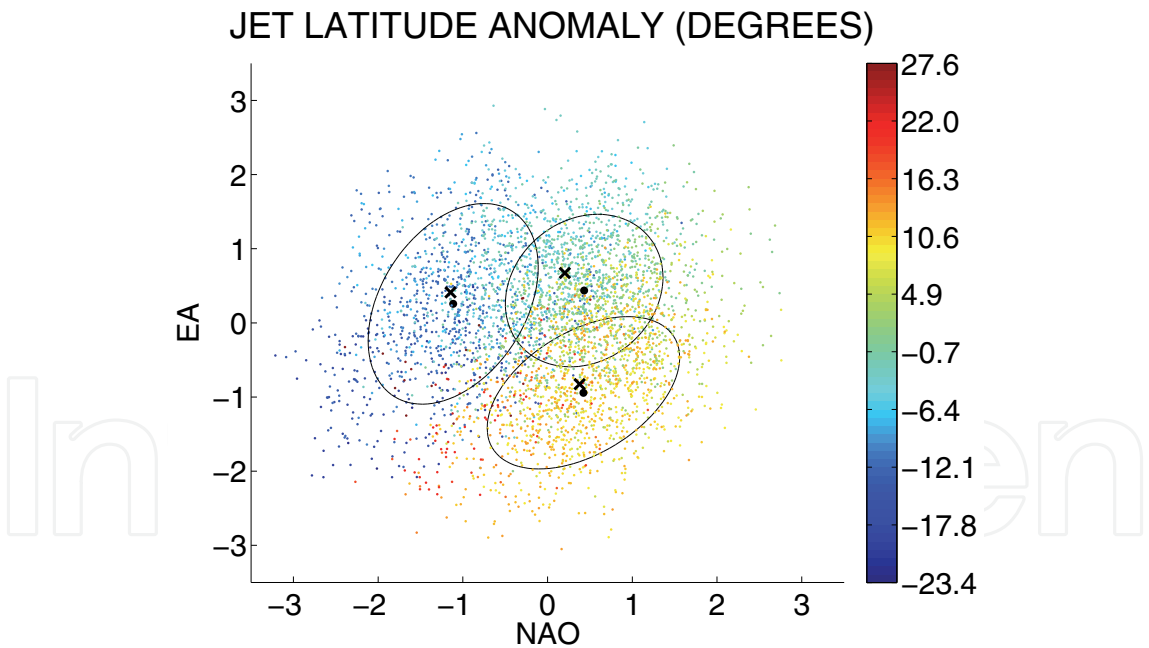
Fig. 6. Scatter plot of the daily winter (DJF) Z500 anomalies, projected onto the NAO/EA plane and color-coded to show the jet latitude. The ellipses and their associated centres correspond respectively to the covariances and the means of the Gaussian component mixture model. The crosses represent the regimes obtained from the jet latitude PDF projected onto the same plane (reproduced from WO10b).
