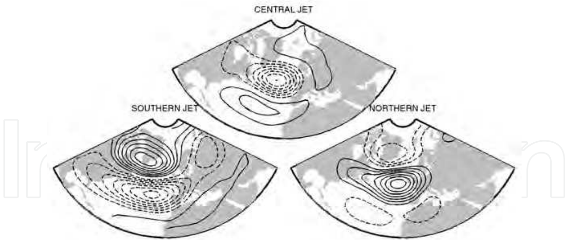
Fig. 5. 500mb geopotential height maps corresponding to the three PDF peaks of the jet latitude. Contour interval 20 m, negative contours dahed and zero contour omitted. Reproduced from WO10b.
