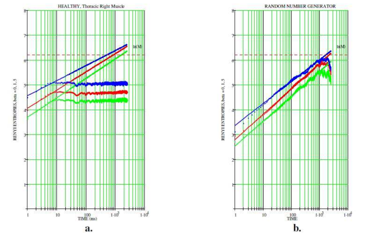
Fig. 1. Entropy vs. \ln t . Top curve \beta = 0 , middle curve \beta = 1 , bottom curve \beta = 5 . a. Subject without LBP for the right thoracic erector spinae muscle; b. Random number generator. The entropy plateau corresponds to the Hurst exponent H \approx 0 . The power spectrum P(f) \sim f^{-\alpha} with an exponent \alpha = 2H + 1 \approx 1 follows P(f) \sim 1/f . Self-organization is generally associated
