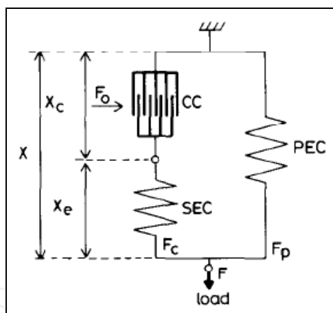
Fig. 3. Schematic diagram of Hill model.
