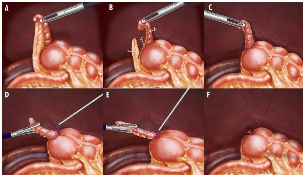
Image 4. Basic technique of laparoscopic appendectomy. (A) exposure of the appendix and meso appendix (B) division of the mesoappendix and appendicular artery (C) isolation of the appendiceal base (D) placement of endoloop at the base of the appendix (E) ligation of the base of the appendix (F) completed appendectomy.
