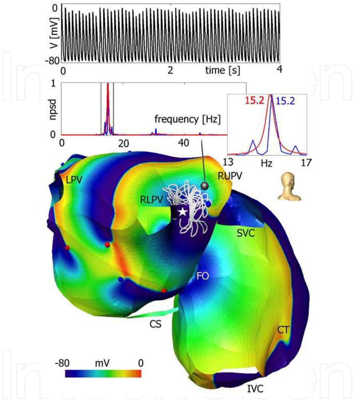
Fig. 3. Snapshot of the action potential after mother rotor anchoring. The atrial model is shown in a posterior oblique view. The mother rotor trajectory is displayed by a white line. Note meandering around the bundle insertion (white asterisk). Spherical markers represent PSs of clockwise (blue) and counter-clockwise (red) chirality. The action potential at a high frequency site (gray marker) is shown together with the power spectrum obtained by the FFT (blue) and the AR-model (red). A portion of the spectrum is zoomed for comparison. CS ... coronary sinus muscle sleeve, CT ... crista terminalis, IVC ... inferior vena cava, FO ... fossa ovalis, LPV ... left pulmonary vein, RLPV ... right lower pulmonary vein, RUPV ... right upper pulmonary vein, SVC ... superior vena cava.
