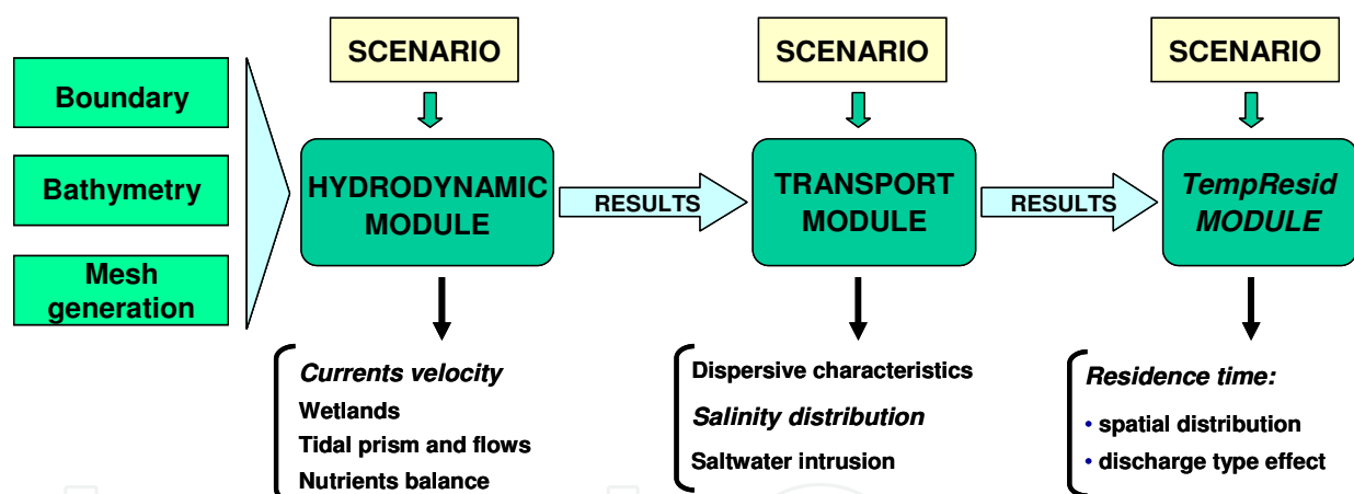
Fig. 13. The MONDEST model conceptualization
