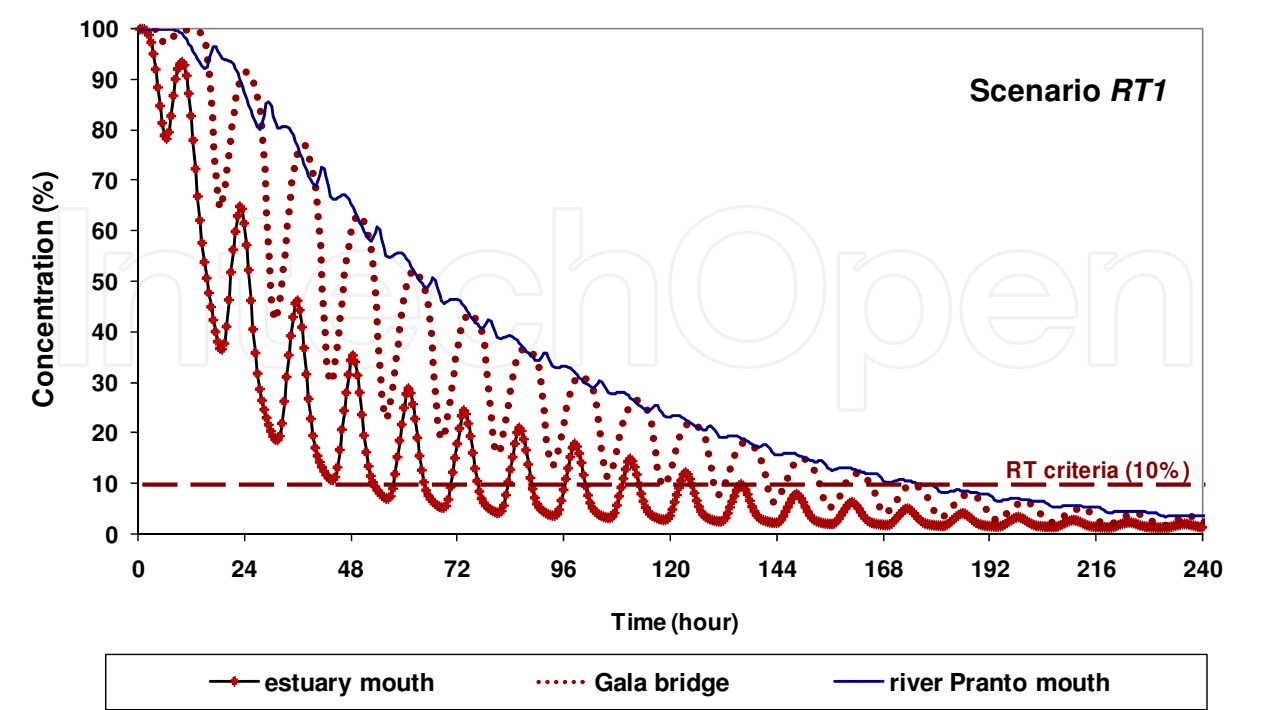
Fig. 15. Residence time computation using TempResid module
