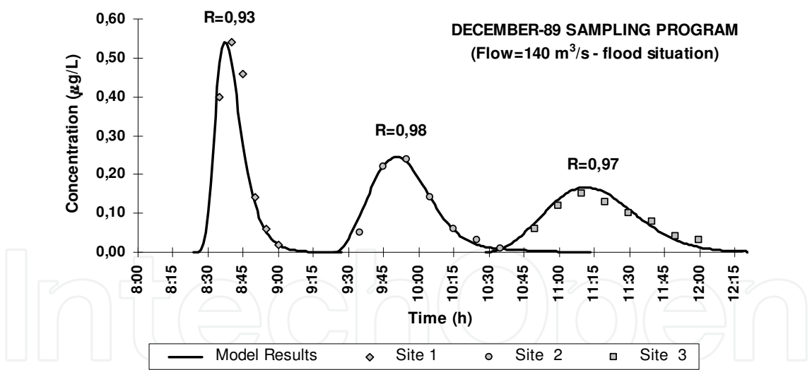
Fig. 12. River Mondego model calibration: correlation between field tracer experiment data and model results.
