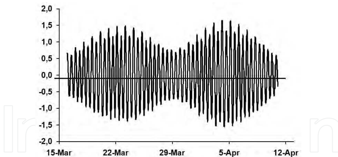
Fig. 9. Monthly tidal harmonic signal at Figueira da Foz harbour using the SR95 programme
