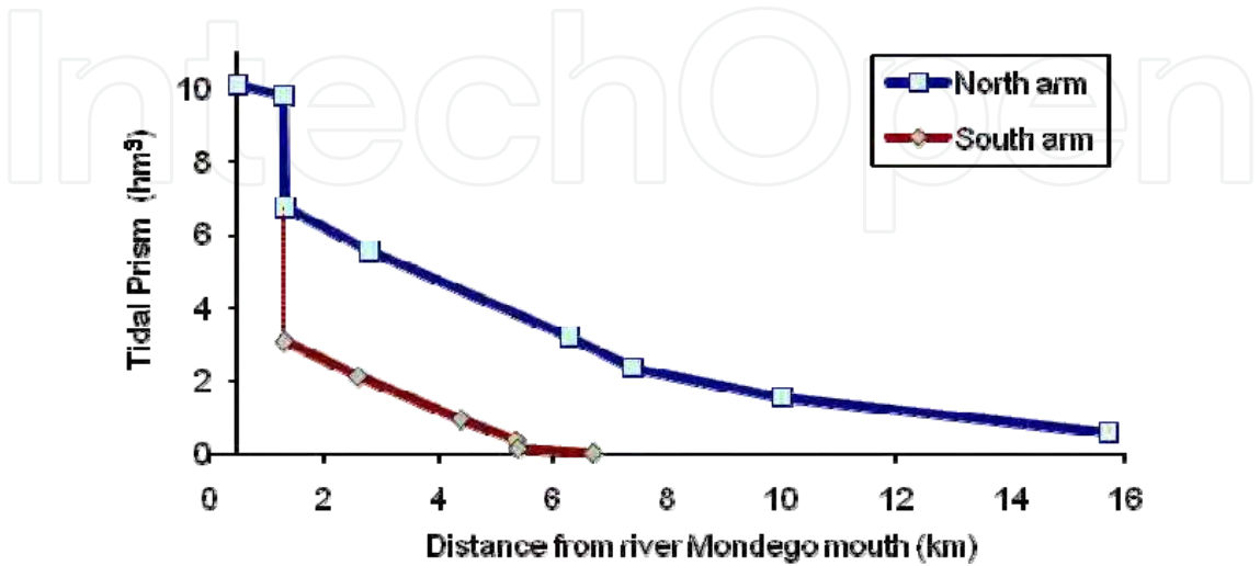
Fig. 19. Tidal prism spatial variation in both estuary arms (flooding of scenario H1)
