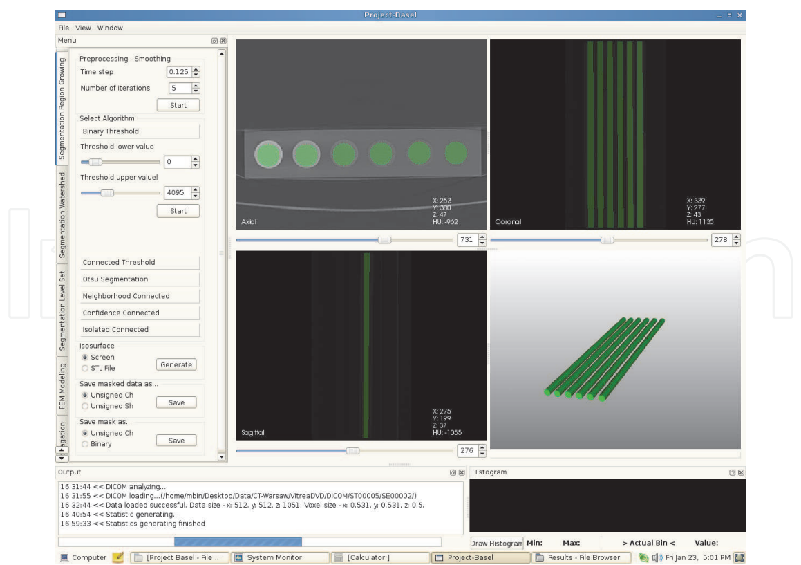
Fig. 4. The density phantom in different views
