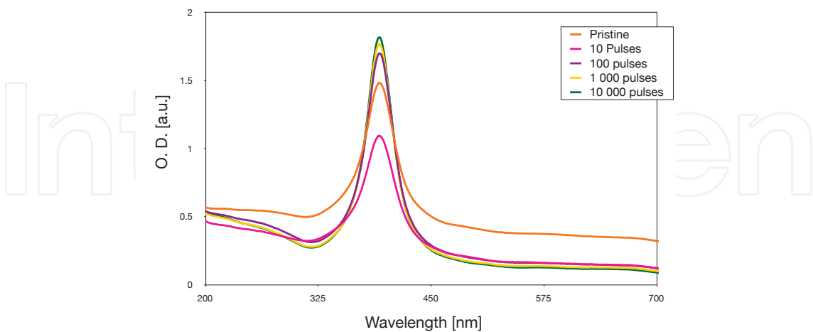
Fig. 7. Effects of infrared laser on Ag nano-particles embedded in SiO 2 : Extinction spectra of samples treated with increasing number of pulses.
