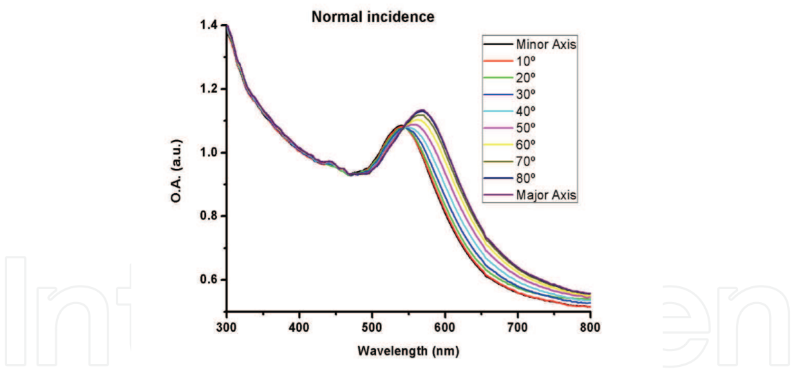
Fig. 5. Extinction spectra of Gold nano-particles in sapphire taken at different polarization angles.
