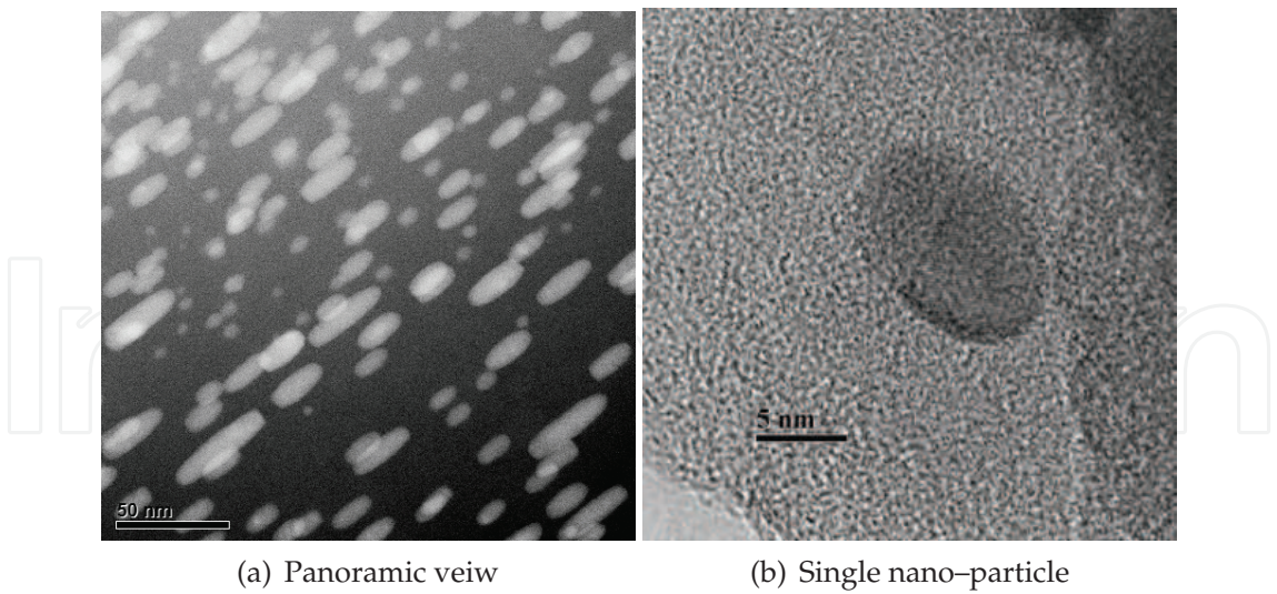
Fig. 4. Electron microscopy images showing the elongation of gold nano-particles by Si ions. (Rangel-Rojo et al. (2010))
