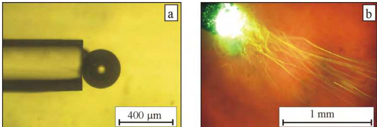
Fig. 5. Laser-induced generation of microbubbles in the vicinity of the blackened end surface of the optical fiber in water for the laser radiation with a wavelength of 0.97\ \mu\text{m} and a power of (a) 1 and (b) 5 W. The photograph is taken from above at an exposure time of 250 ms.
