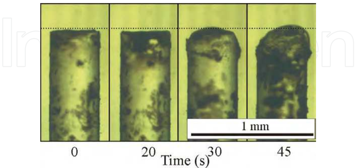
Fig. 12. Modifications of the profile of the blackened fiber tip surface (side view) for regime of channel formation (the channel is formed by the fiber that moves inside the wooden bar with water and the radiation power is 5 W). The left-hand panel shows the original fiber just after its blackening (Yusupov et al., 2011a).
