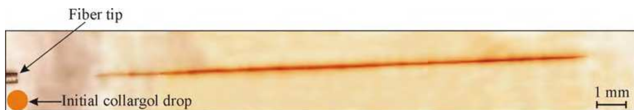
Fig. 18. Micro-image (in transmission mode) of filament of Ag nanoparticles fabricated in water nearby optical fiber tip at 2.5 W of laser power (Yusupov et al, 2011b).
