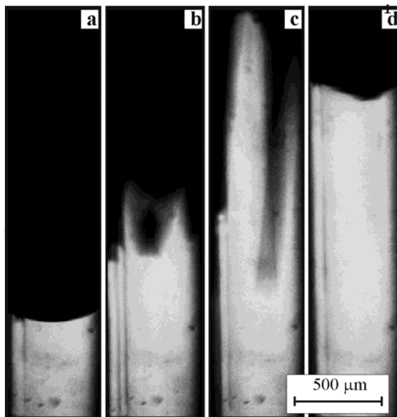
Fig. 9. Variation of a meniscus shape in a capillary caused by laser induce hydrodynamics and bubbles formation. Laser wavelength is 1.56\ \mu\text{m} , laser power – 1\text{W} , internal diameter of capillary – 500\ \mu\text{m} .
