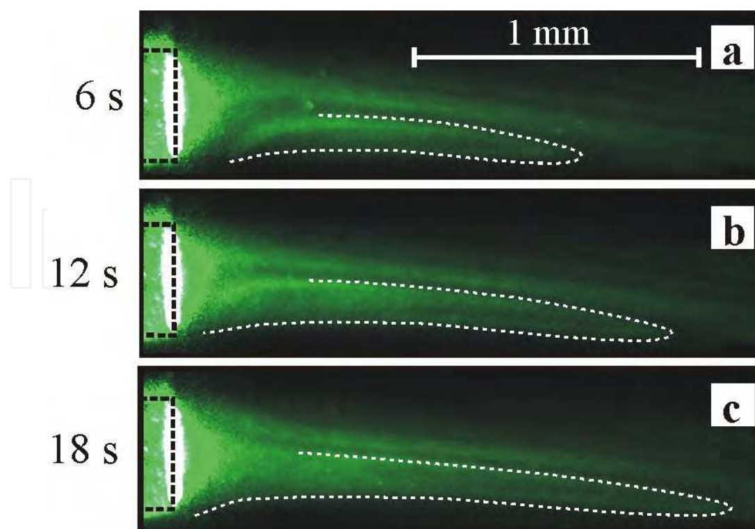
Fig. 4. Microscope pictures (in scattering mode) of intrusions of Ag nanoparticles in water (outlined with dashed line) stimulated by laser induced hydrodynamics nearby optical fiber tip at 1.0 W of 0.97 \mu\text{m} laser power in 6 s (a), 12 s (b), and 18 s (c) of laser irradiation. Fiber tip is shown by dashed line (Yusupov et al., 2011b).
