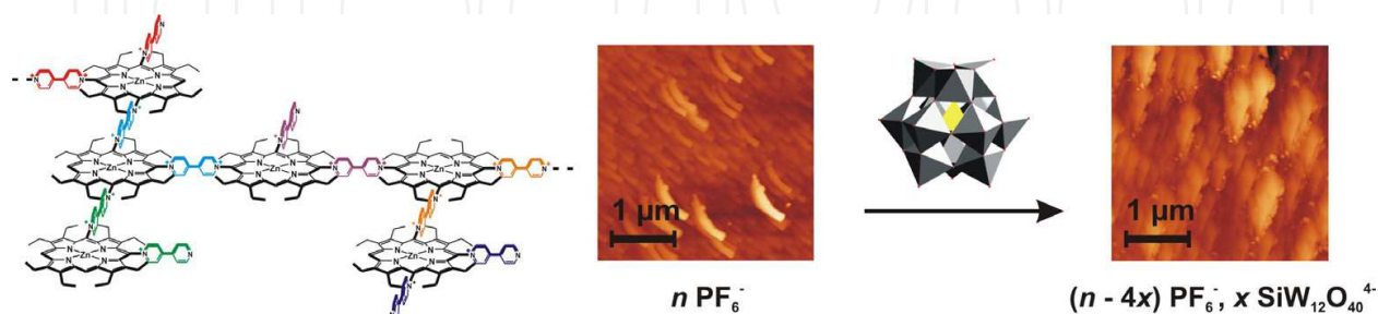
Fig. 22. Atomic force micrographs of an ITO electrode coated with the polymer obtained from 5,10-ZnOEP(bpy) 2 2+ after plunging for 10 hours in water (left) and in a solution of SiW 12 O 40 4- (1 mM) (right).
