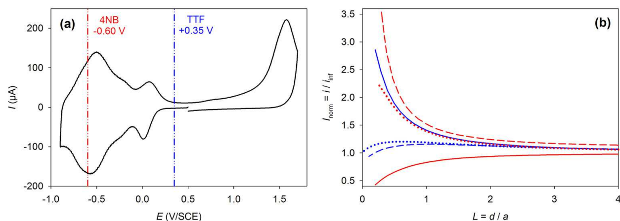
Fig. 12. (a) Cyclic voltammogram of the polymer obtained from ZnOEP and bpy after 25 iterative scans onto ITO electrode in \text{CH}_3\text{CN} and 0.1 \text{ M NBu}_4\text{PF}_6 ( v = 0.2 \text{ V s}^{-1} ), with indications of the redox potential values of several mediators used. (b) SECM approach curves, in \text{CH}_3\text{CN} and 0.1 \text{ M NBu}_4\text{PF}_6 on non-coated ITO electrodes (full lines), ITO electrodes coated with the polymer obtained from ZnOEP(bpy) + after 25 iterative scans (dashed lines) and ITO electrodes coated with the polymer obtained from ZnOEP and bpy after 25 iterative scans (dotted lines), with TTF (—) and 4NB (—) used as redox mediators. L is the normalized distance and I_{\text{norm}} is the normalized current, where i corresponds to the current at a platinum microelectrode (with a radius a equal to 5 \mu\text{m} ) localized at a distance d from the substrate and i_{\text{inf}} corresponds to the steady-state current when the microelectrode is at an infinite distance from the polymeric substrate.
