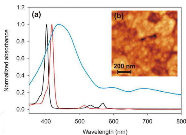
Fig. 15. (a) Normalized UV-visible absorption spectra of ZnOEP in 1,2- \text{C}_2\text{H}_4\text{Cl}_2 (—), of 5,15- \text{H}_2\text{Py}_2\text{Ph}_2\text{P} in 1,2- \text{C}_2\text{H}_4\text{Cl}_2 (—), and of an ITO electrode modified with the copolymer obtained from ZnOEP and 5,15- \text{H}_2\text{Py}_2\text{Ph}_2\text{P} after 25 iterative scans (—). (b) Atomic force micrograph of the same copolymer after washing with water.
