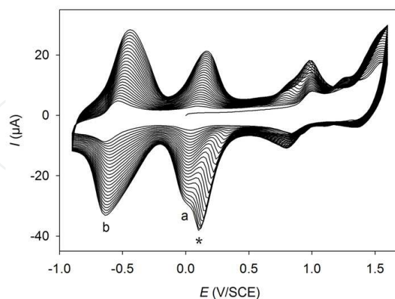
Fig. 4. Cyclic voltammograms recorded during the iterative scans between -0.90 and +1.60 V/SCE of ZnOEP(bpy) + (0.25 mM) in 1,2-C 2 H 4 Cl 2 and 0.1 M NEt 4 PF 6 . Working electrode: ITO; S = 1 cm 2 ; v = 0.2 V s -1 .
