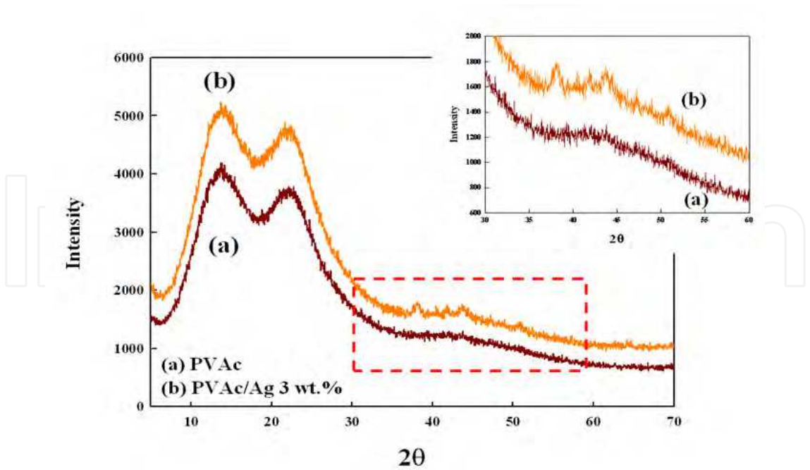
Fig. 4. XRD patterns of (a) pure PVAc and (b) PVAc/Ag nanocomposite microparticles with surfactant
