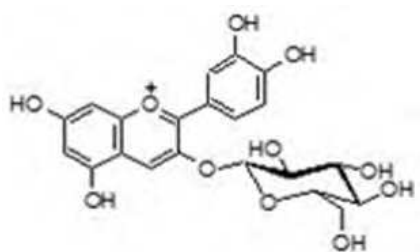
Fig. 17. Chemical structure of Cyanidin-3-O-glucoside
