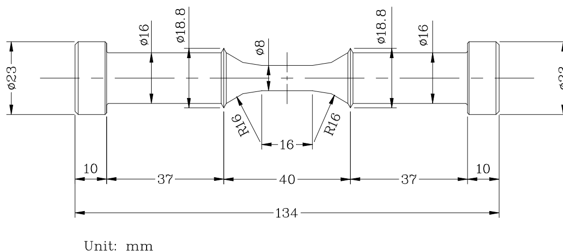
Fig. 1. Round bar specimen for low-cycle fatigue test.
