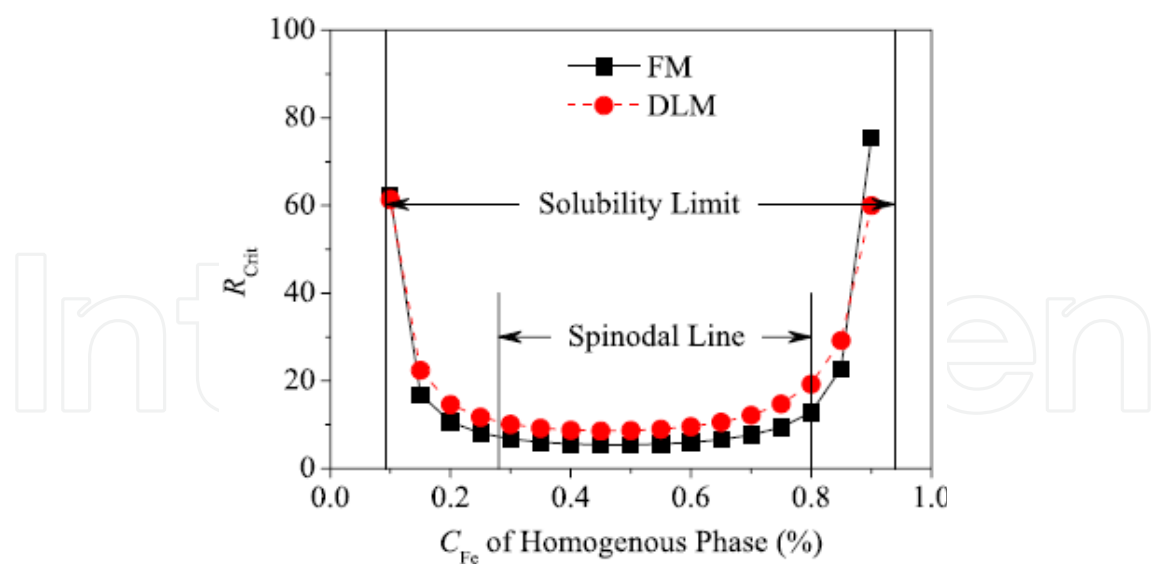
Fig. 7. Critical nucleus size ( R_{crit} in Å) as a function of the composition of the homogenous phase Fe_cCr_{1-c} for ferromagnetic and paramagnetic states. The vertical lines show the experimental spinodal and solubility limits.
