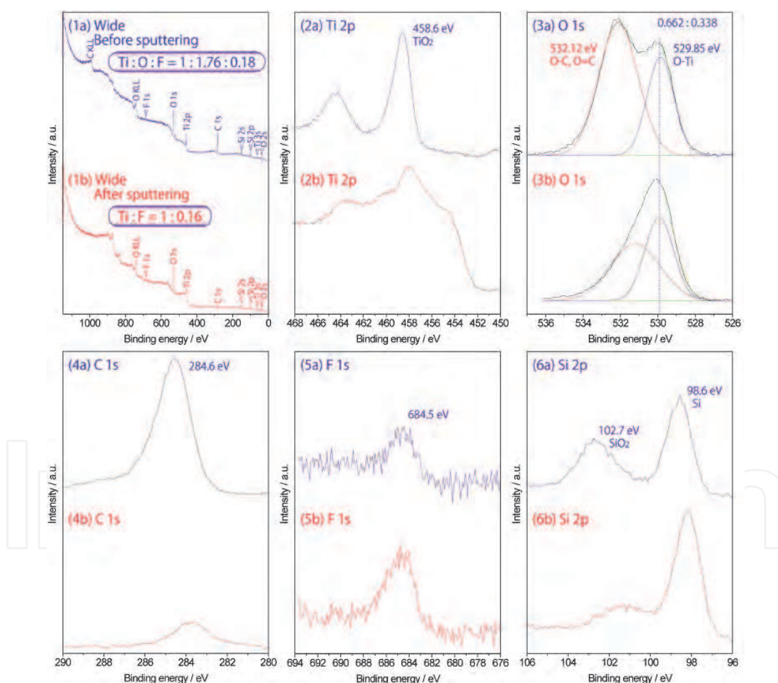
Fig. 24. XPS spectra of (1) wide scan, (2) Ti 2p, (3) O 1s, (4) C 1s, (5) F 1s and (6) Si 2p for a micro-structured substrate coated with the multi-needle TiO 2 particles deposited for 7d (a) before and (b) after Ar + sputtering. (3a) O1s spectra decomposed to two peaks after removal of background. Reprinted with permission from Ref. 121 , Masuda, Y., Ohji, T. and Kato, K., 2010, Cryst. Growth Des. , 10, 913. Copyright ©American Chemical Society
