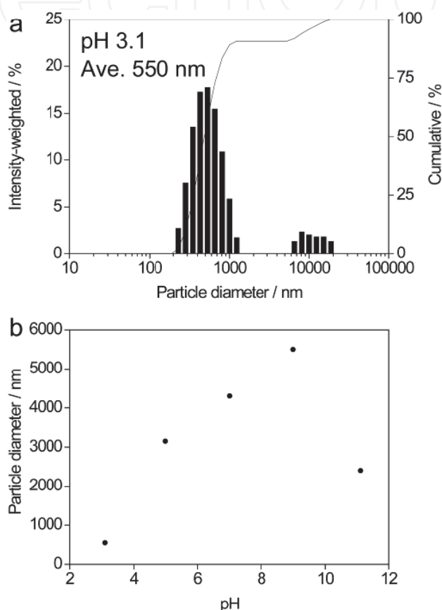
Fig. 19. (a): Particle size distribution of anatase TiO 2 particles at pH 3.1. (b): Particle size of anatase TiO 2 particles as a function of pH. Reprinted with permission from Ref. 77 , Masuda, Y. and Kato, K., 2008, Cryst. Growth Des. , 8, 3213. Copyright ©American Chemical Society
