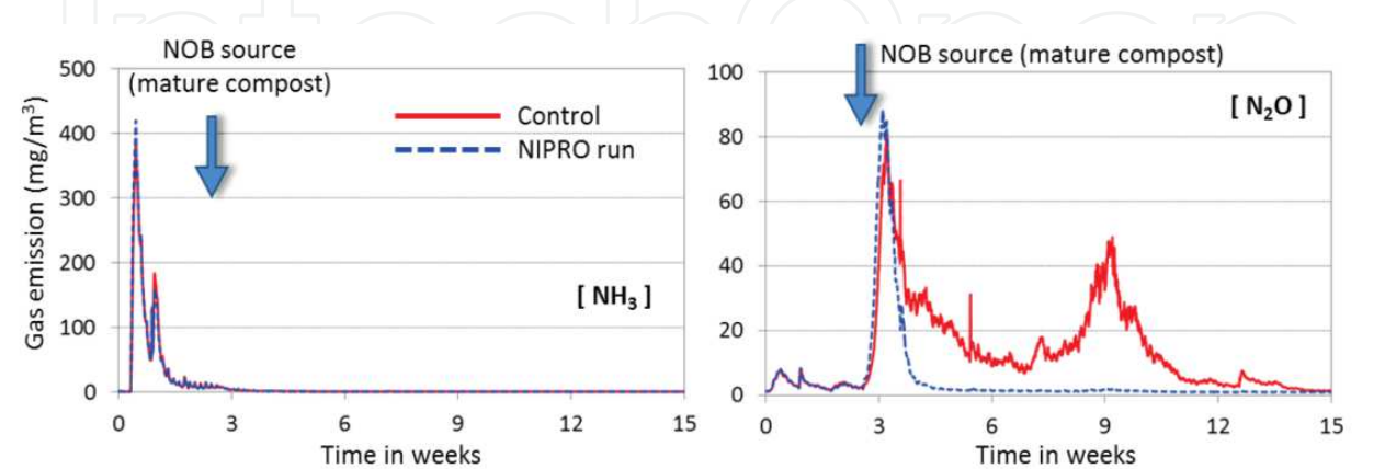
Fig. 7. Emission patterns of \text{NH}_3 and \text{N}_2\text{O} during swine manure composting. Arrow indicates addition of NOB source of mature swine compost
