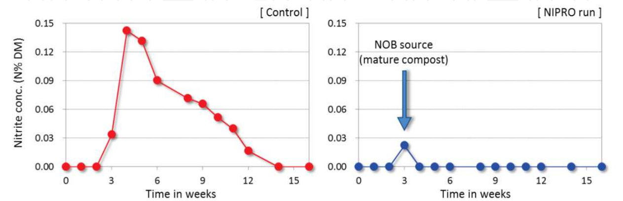
Fig. 3. Changes in concentration of nitrite nitrogen during swine manure composting. Arrow indicates addition of NOB source of mature swine compost
