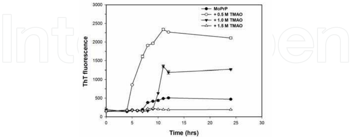
Fig. 8. Kinetic traces for amyloid fibril formation from MoPrP monitored by ThT-binding fluorescence in the presence of 2 M GdnHCl and various concentrations of TMAO at pH 6.0 at 37 °C. The fluorescence readings were average values of two measurements
