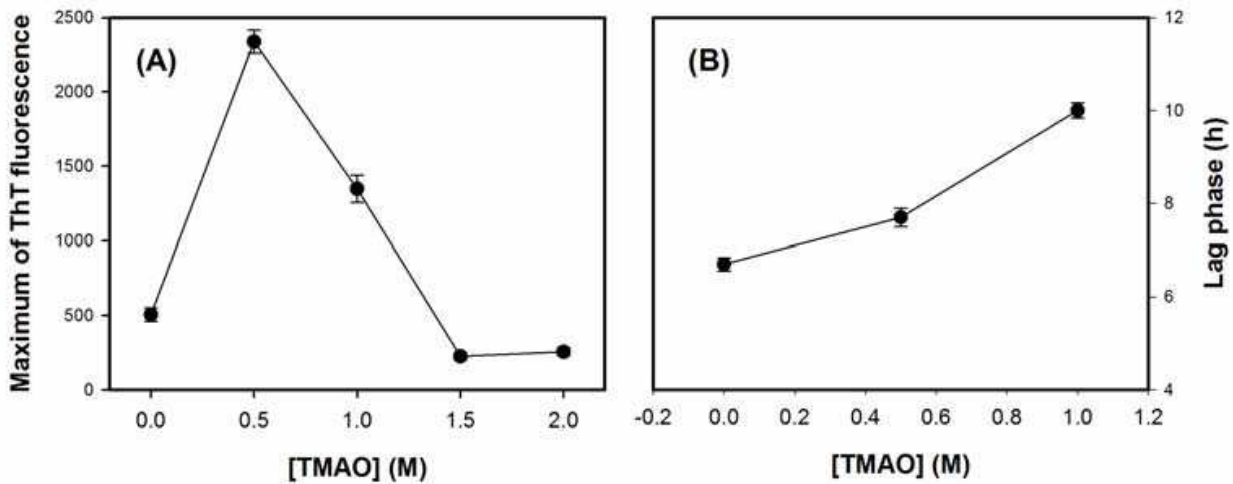
Fig. 9. (A)The quantity of amyloid fibrils converted from MoPrP monitored by the maximum of ThT-binding fluorescence measured two times, and (B) the calculated lag phase of fibril conversion in the absence and in the presence of TMAO
