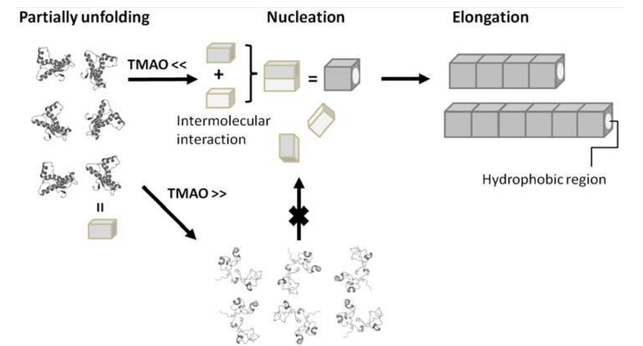
Fig. 13. A scheme illustrating the proposed effect of TMAO based on nucleation-dependent polymerization model
