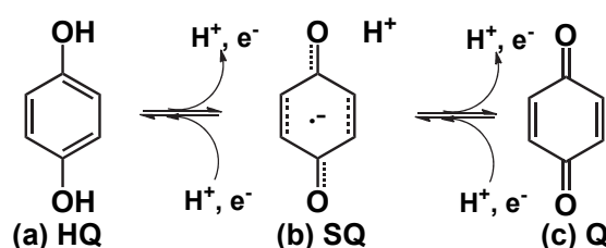
Fig. 1. Proton-coupled electron transfer in hydroquinone molecules
