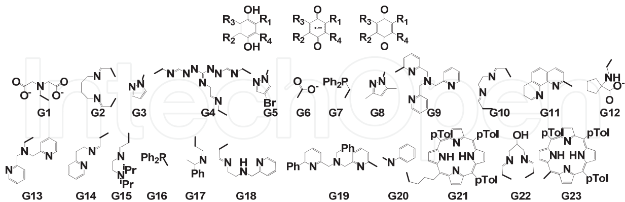
Fig. 3. Substituents of hydroquinone / p -semiquinone / p -quinones used for transition metal ion ligation
