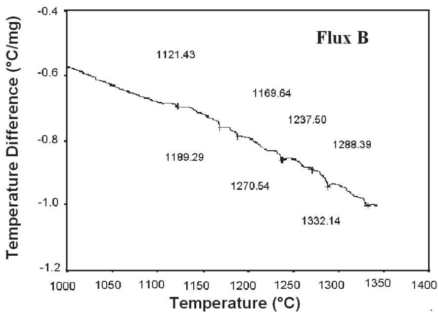
Fig. 6. DTA diagram of flux B.
