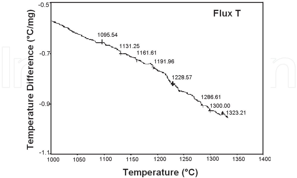
Fig. 8. DTA diagram of flux T.
