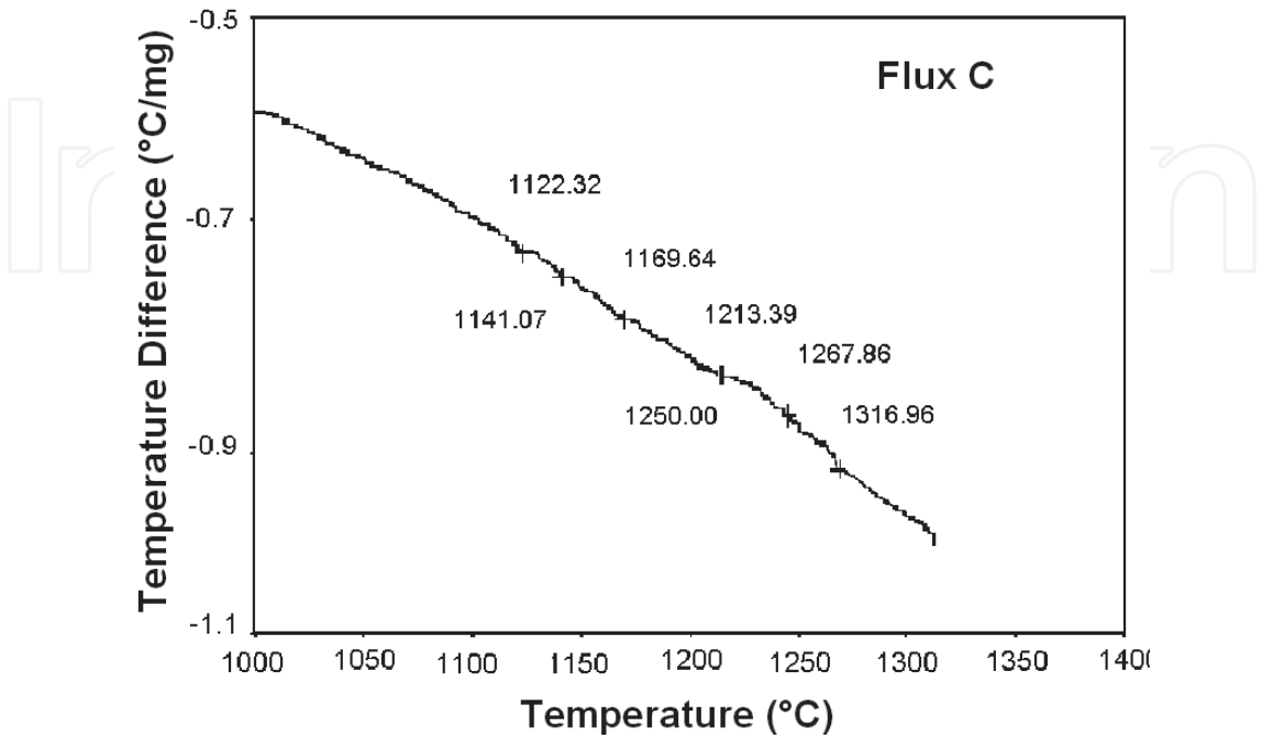
Fig. 7. DTA diagram of flux C.
