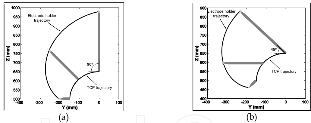
Fig. 6. Tool Center Point and electrode holder trajectories for 90° (a) and 45° (b) welding angles in orbital welding.
