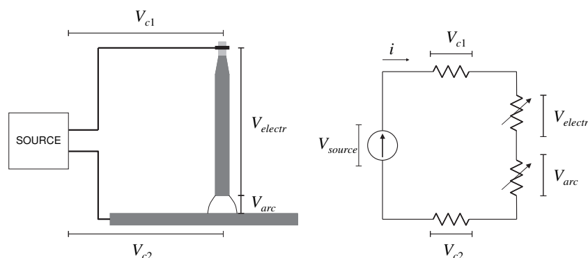
Fig. 7. Electrical circuit of covered electrode welding
