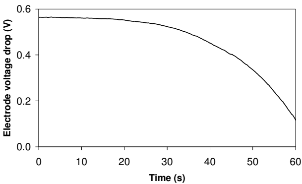
Fig. 9. Electrode voltage drop during welding.
