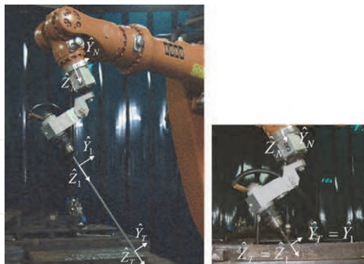
Fig. 8. Complete electrode and melted electrode frames.
