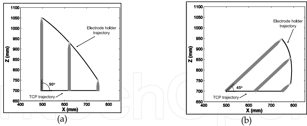
Fig. 5. Tool Center Point and electrode holder trajectories for welding angles of (a) 90° and (b) 45°.
