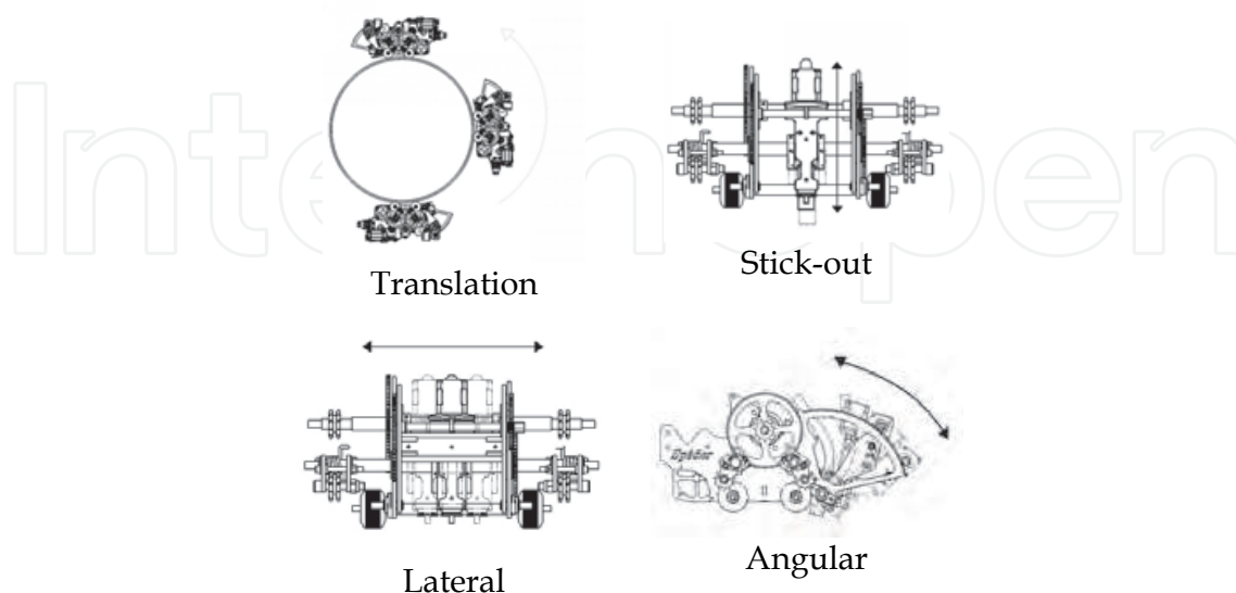
Fig. 31. Degrees of freedom of the robot.
