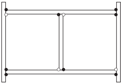
Fig. 25. Arc spot welds configuration to increase flexural stuffiness resistance using only 8 spots.
