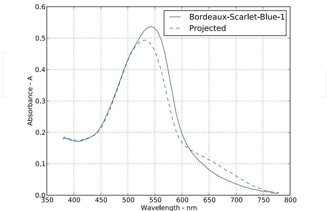
Fig. 14. Combined Spectrum of Bordeaux, Scarlet and Blue-1 Direct Dyes
