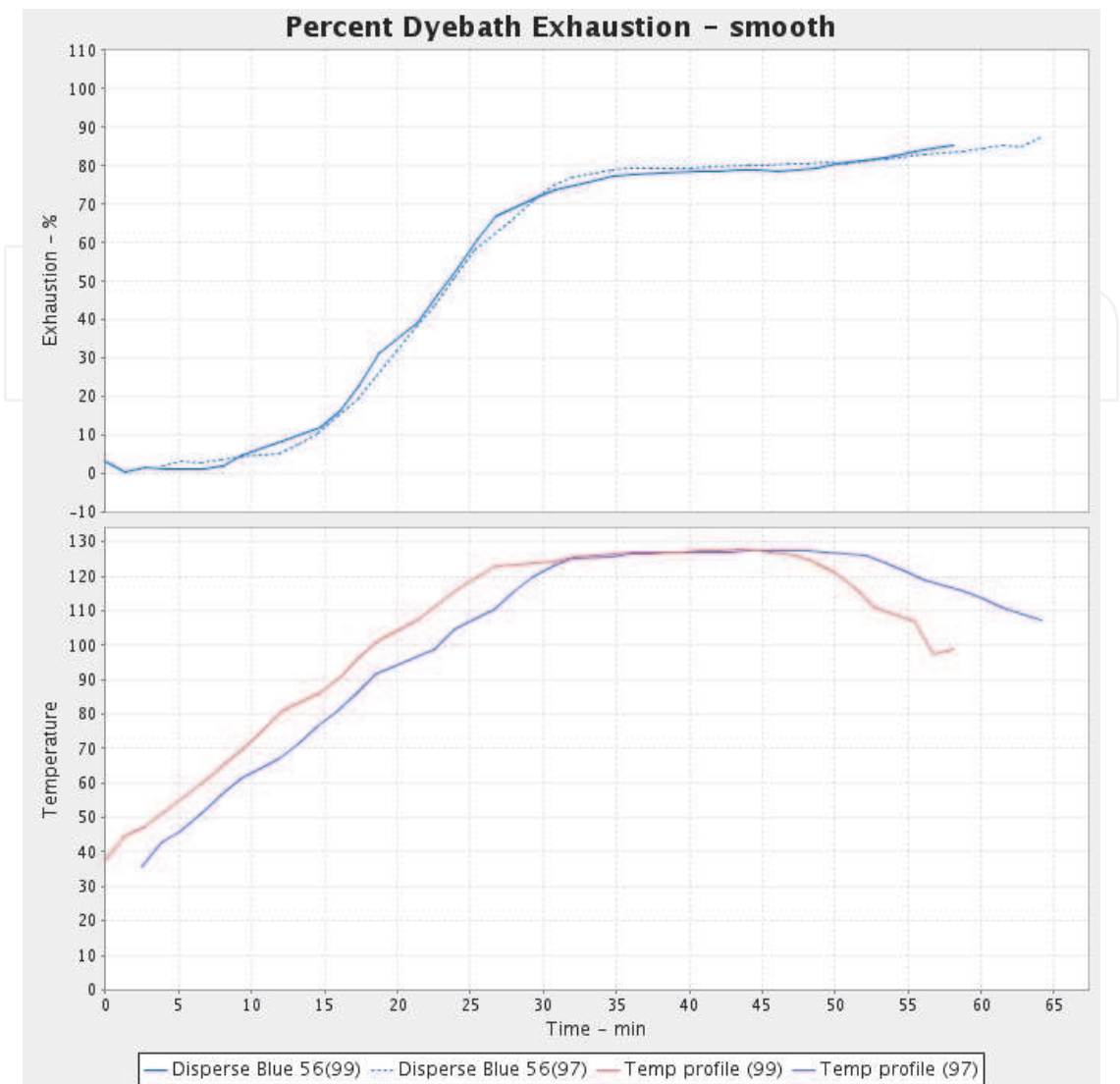
Fig. 9. Different yarn used in same fabric structures.
