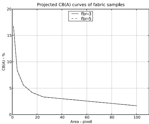
Fig. 22. Theoretically projected CB(A) curves
