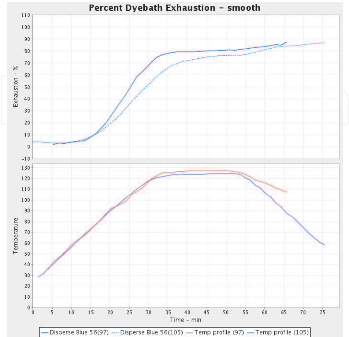
Fig. 10. Same yarn used in different fabric structures.
