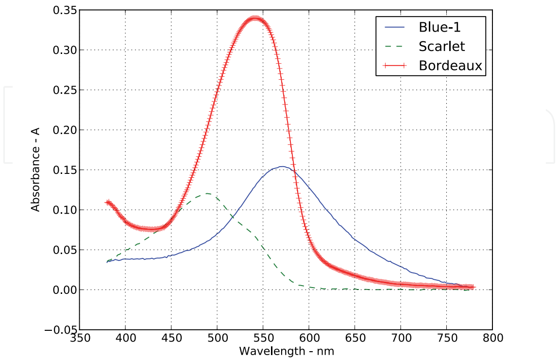
Fig. 13. Spectra of 3 different direct dyes
