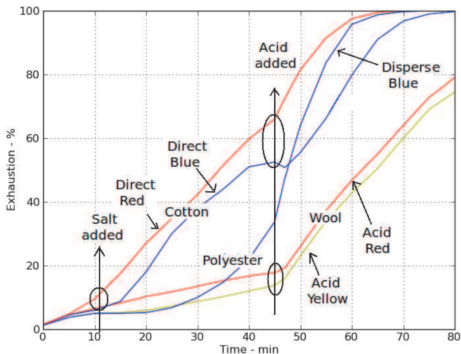
Fig. 2. The monitoring of dye uptake by the fabric for individual dyes during a dyeing cycle. Regardless of the choice to run in manual or automatic mode, a micro sample is enough to calculate the individual dye amounts in the solution. This data may then be correlated with the temperature, pH, and conductivity sensor measurements if they are attached. The results are then presented to the dyer in real-time at various overlay graphs. When the dyeing is completed, the technician may save the results in a database. The data stored may then be analyzed by an engineer following the methodology suggested in this paper.
