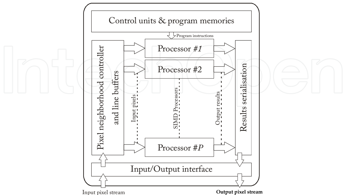
Fig. 3.2. A P processors computing tile.
