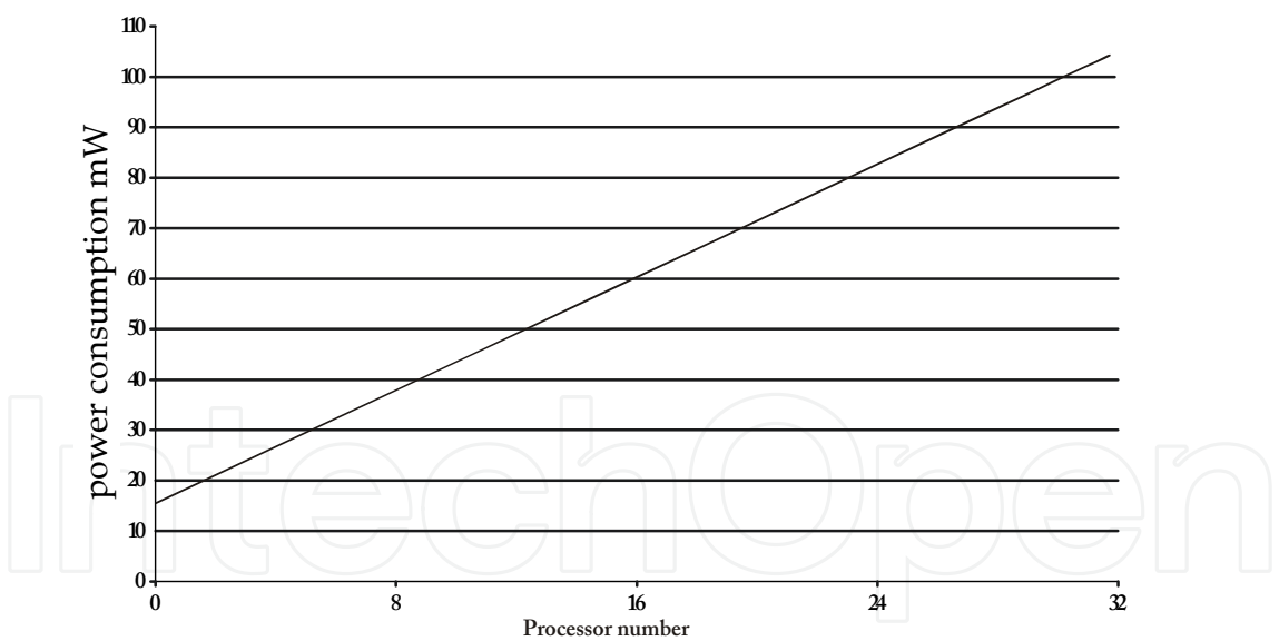
Fig. 3.3. Characterization of the power consumption of a single computing tile eISP architecture versus number of processors.
