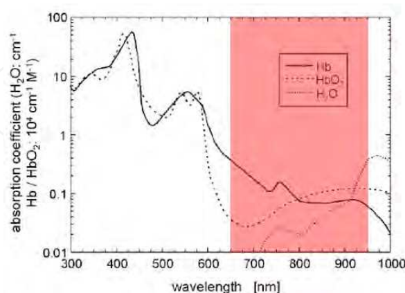
Fig. 2. The optical window between 650 and 950 nm, where absorption by water haemoglobin and deoxyhaemoglobin is minimal.
