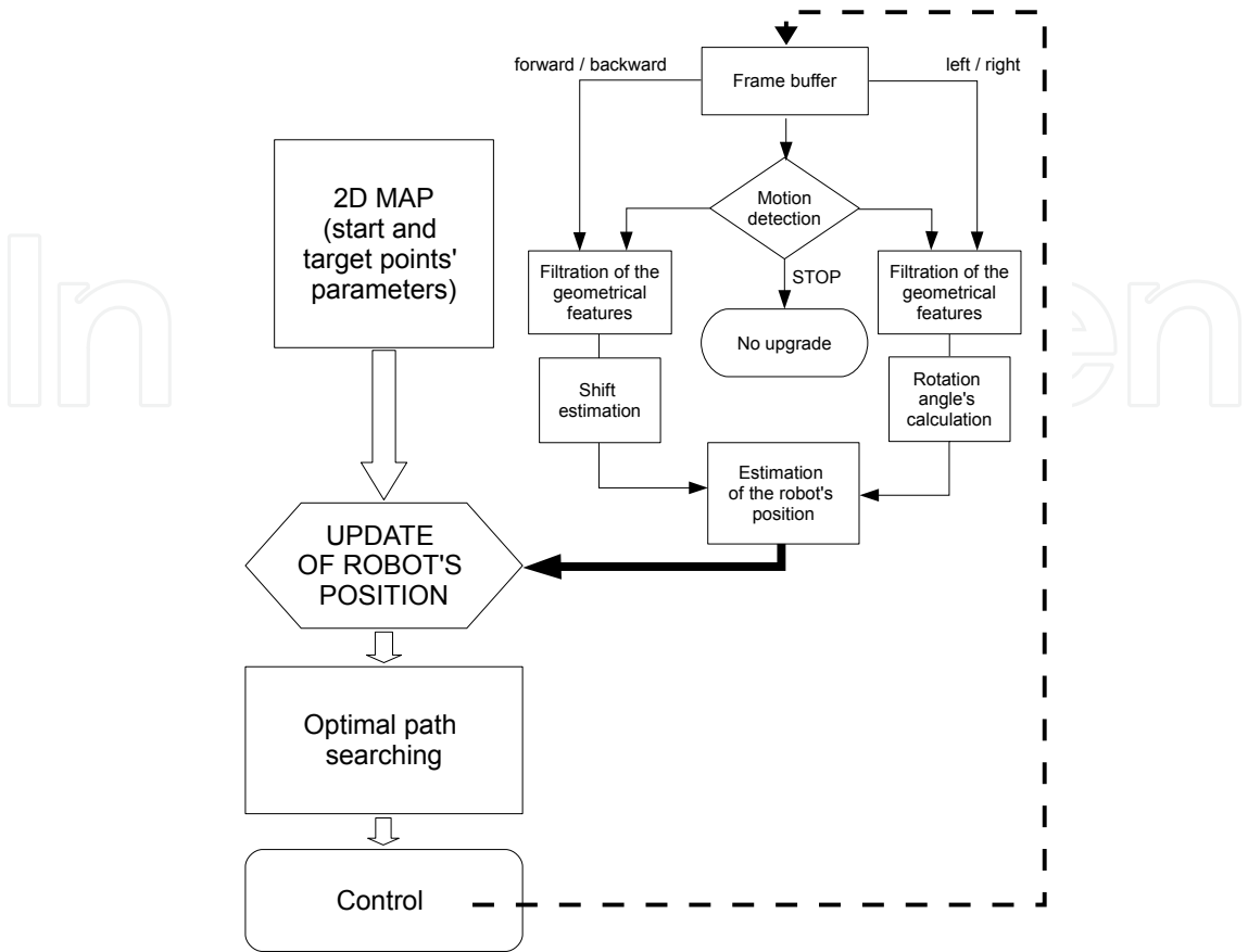
Fig. 2. Illustration of the general vision based control algorithm of the mobile robot
