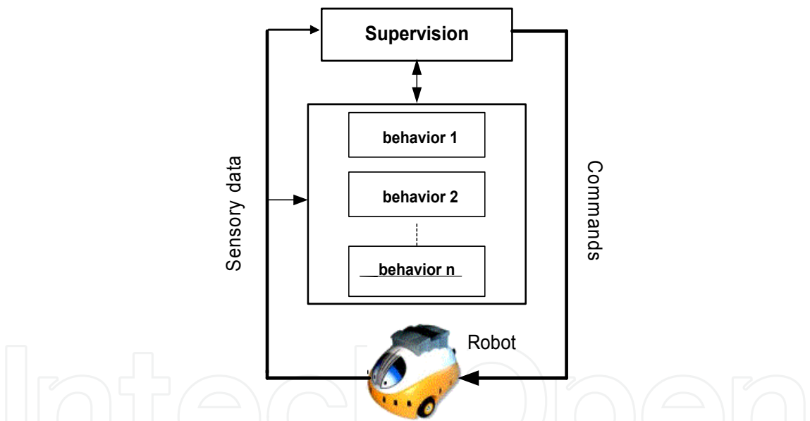
Fig. 5. Architecture of Context Dependent Behavior Coordination.
