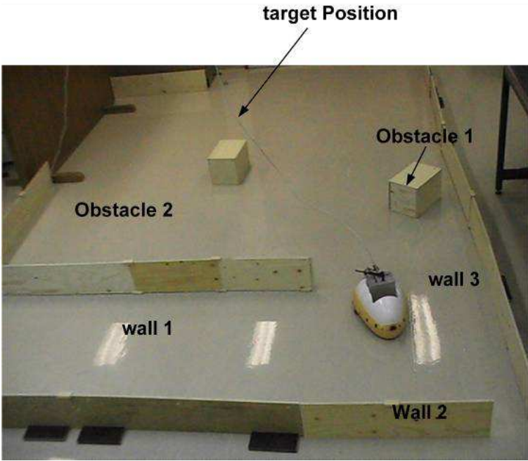
Fig. 24. Pekkee Navigates in a crowded environment.
