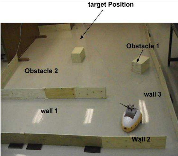
Fig. 23. Pekkee Navigates in a crowded environment.
