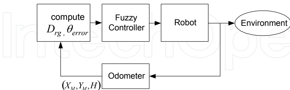
Fig. 6. Control architecture for goal reaching Behavior.
