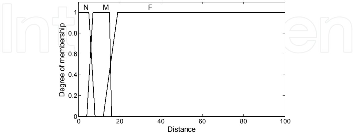
Fig. 9. Input membership function for distance to obstacle, N:Near, M:Medium, F:Far
