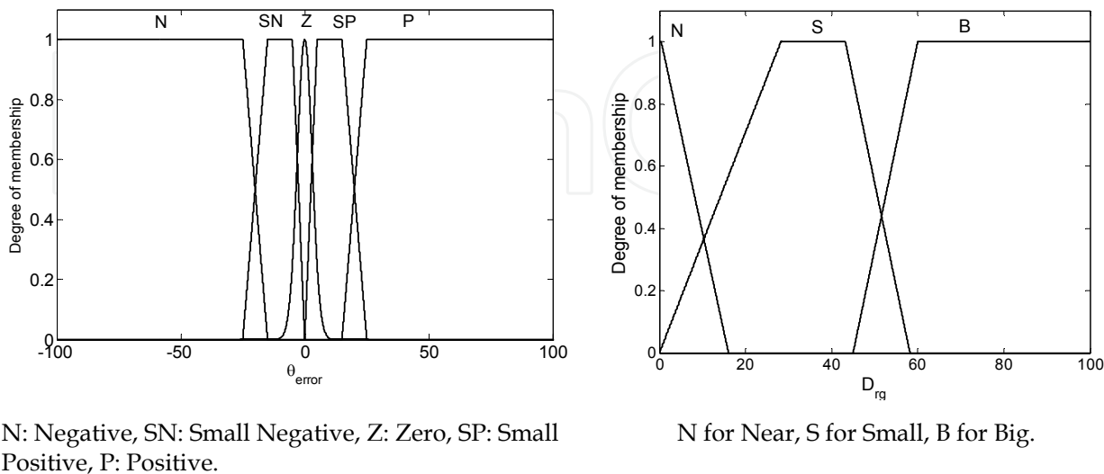
Fig. 7. Input membership functions for D_{rg} and \theta_{error} .
