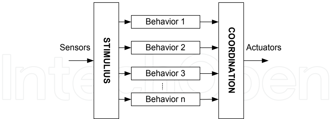
Fig. 3. Structure of behavior based navigation.
