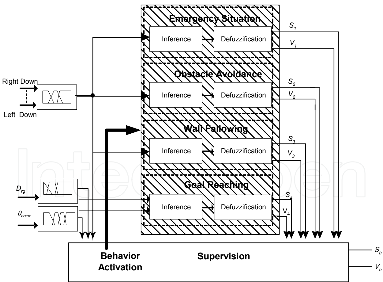
Fig. 11. Supervision Architecture.
