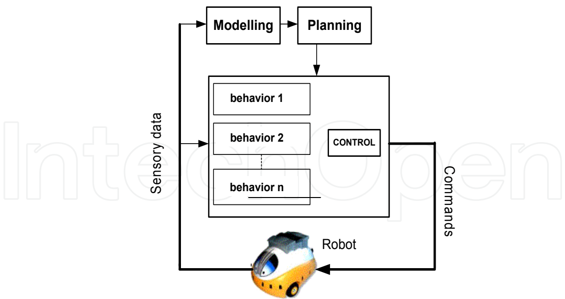
Fig. 4. Architecture of compared method.
