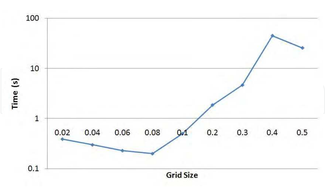
Fig. 18. The effect of grid size on computation time.
