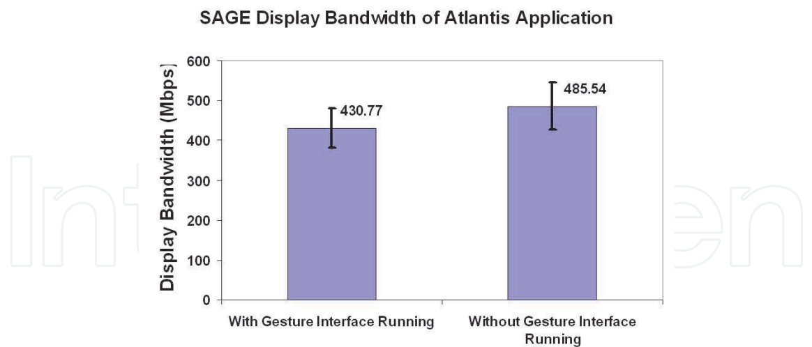
Fig. 8. Display bandwidths of the SAGE middleware, with and without the gesture interface running.
