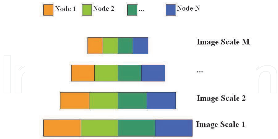
Fig. 3. Illustration of the by-region task partitioning strategy.
