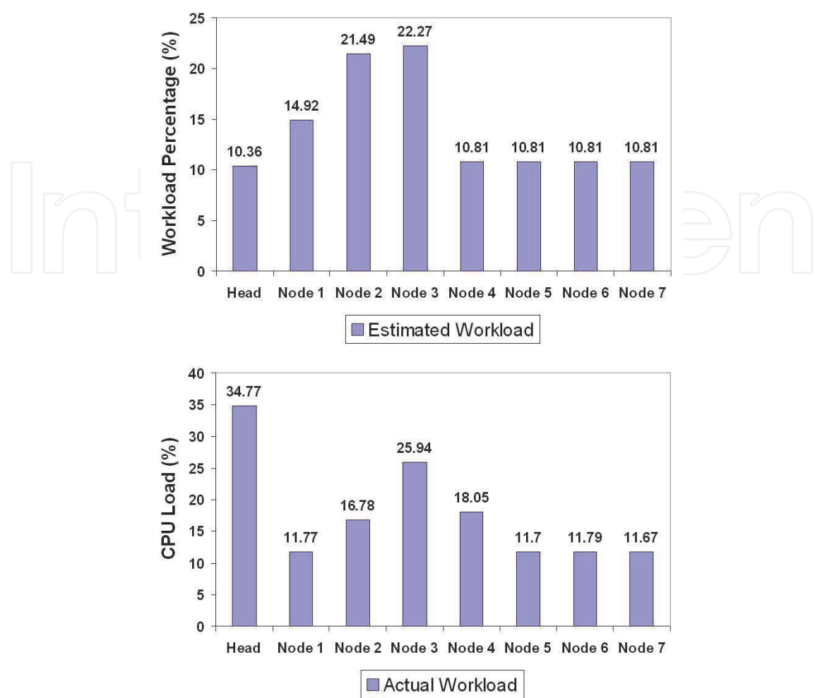
Fig. 7. Estimated and actual workload distributions across a 8-node scanning tree. Note that the units used by top and bottom plots are different.
