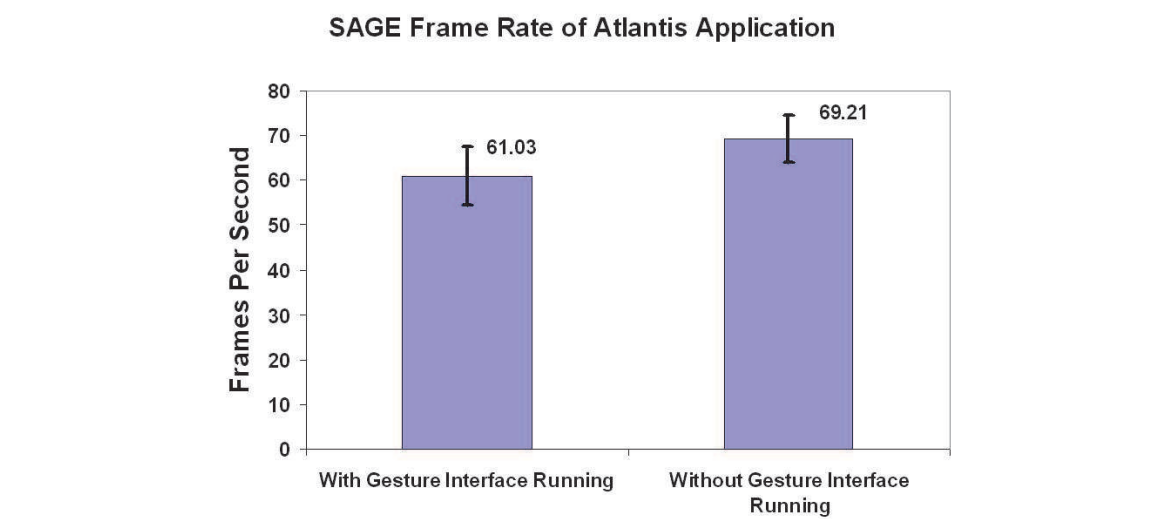
Fig. 9. Frame Rates of the SAGE middleware, with and without the gesture interface running.
