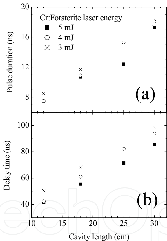
Fig. 6. Cr:Forsterite laser characteristics of the pulse duration (a) and delay time (b) with the cavity length of 12–30 cm. The Cr:Forsterite laser energy was 3 mJ, 4 mJ, and 5 mJ.
