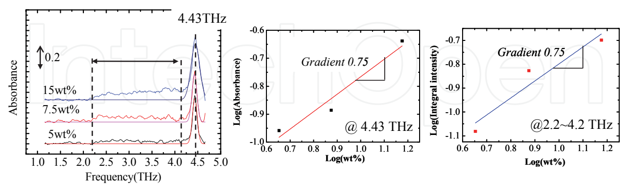
Fig. 11. THz spectra of Cu 2 O with various concentrations at room temperature.
