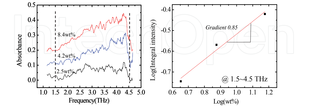
Fig. 12. THz spectra of CuO with various concentrations at room temperature.
