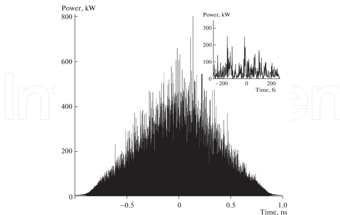
Fig. 8. Numerically simulated plot of the SC radiation intensity vs time. The inset shows a fragment of the time distribution on a smaller scale.
