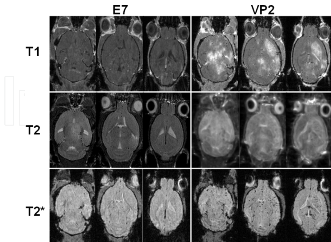
Fig. 7. In vivo MRI images of 8 day TMEV infected C57BL/6 mice, 24 hours after VP2 121-130 peptide injection (right panel) or irrelevant E7 peptide injection (left panel). Top row: axial images extracted from the gadolinium enhanced T1 weighted dataset demonstrate extensive contrast enhancement of confluent areas of the brain in the VP2 injected mouse, and very faint enhancement in the parahippocampal area in the E7 injected animal. Middle row: T2 weighted images demonstrate T2 hyperintensities, corresponding with areas of edema, inflammatory infiltrates, demyelination and tissue damage in the VP2 injected mouse; minimal hyperintense changes are also demonstrated in the parahippocampal areas of the E7 injected animal. Bottom row: T2* weighted images demonstrate punctuate T2 hypointensities, corresponding with areas of microhemorrhages in the VP2 injected mouse. (Reproduced with permission from Pirko, I., G. L. Suidan, et al. (2008). Acute hemorrhagic demyelination in a murine model of multiple sclerosis. Journal of neuroinflammation 5: 31).
