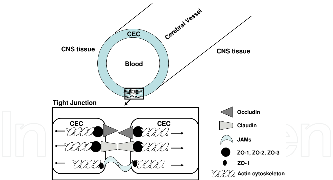
Fig. 2. Molecular model of tight junctions between cerebral endothelial cells (CECs). Occludins, claudins and junctional adhesion molecules (JAMs) regulate adhesion of CECs. Occludins and claudins adhere to the zona occludin complex which consists of an interaction of ZO-1, ZO-2, and ZO-3 proteins. In contrast JAMs adhere only to zona occludin-1 (ZO-1). The zona occludin proteins in turn adhere to actin cytoskeleton proteins. Opening of tight junctions during inflammation appears to be an orchestrated event of degradation and expression of occludins and claudins, respectively and contraction of actin cytoskeleton. Model is modified from (Minagar & Alexander, 2003).
