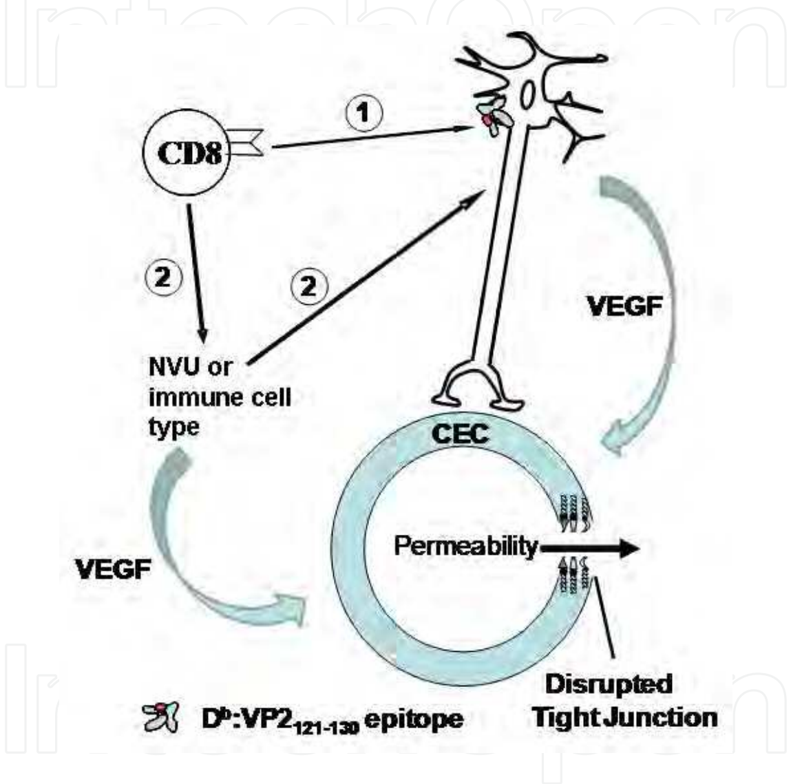
Fig. 10. BBB disruption in the PIFS model is induced through intravenous injection of VP2 121-130 peptide at 7 days post TMEV infection. At 7 days post TMEV infection, the CNS infiltrating D b :VP2 121-130 specific CD8 T cell response peaks. Administration of VP2 121-130 peptide results in heightened activation of expanded CNS infiltrating D b :VP2 121-130 specific CD8 T cells interacting with D b class I expressing cells, which could include neurons, astrocytes, cerebral endothelial cells, pericytes and microglia. Our central hypothesis (1.) is that CD8 T cells engage neurons to promote upregulation of VEGF. Our alternative hypothesis (2.) is that CD8 T cells engage a different CNS cell type that results in BBB disruption and vascular permeability that is dependent or independent of neuronal VEGF.
