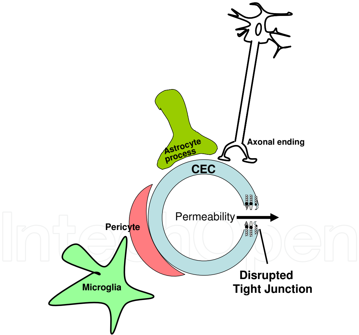
Fig. 1. A model depicting the organization of the neurovascular unit (NVU). The NVU is composed of cerebral endothelial cells (CECs) surrounded by astrocytes, pericytes, axonal endings, and microglia. The NVU may ultimately control permeability of the BBB through tight junctions between CECs of the vasculature.
