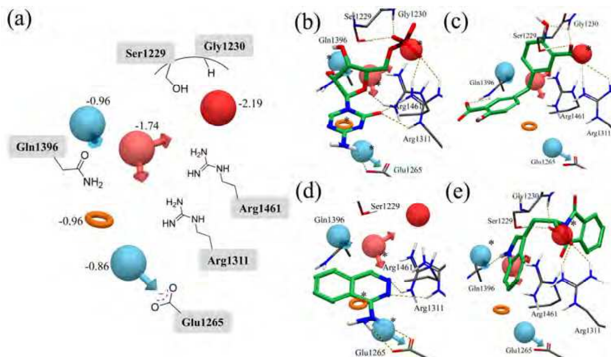
Fig. 5. (a) Structure-based pharmacophore model proposed for human DNMT1 inhibitors. Red sphere: negative ionizable, pink sphere: hydrogen bond acceptor, blue sphere: hydrogen bond donors, and orange ring: aromatic ring. Selected amino acid residues in the catalytic site of homology model are schematically depicted for reference. Comparison between the binding mode and pharmacophore hypothesis for representative DNMT inhibitors, (b) 5-azacytidine, (c) NSC14778, (d) hydralazine, and (e) RG108.
