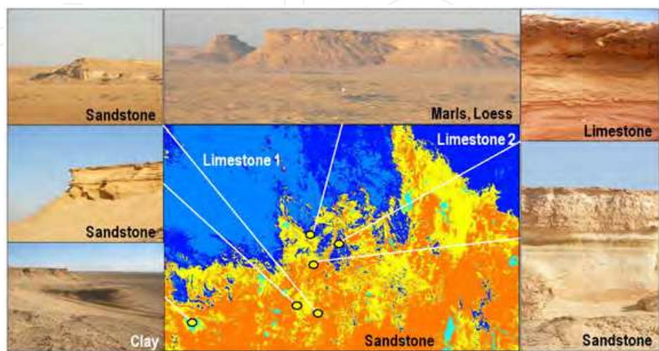
Fig. 10. Validation of lithology map in the field [after Coulson et al. 2009]
