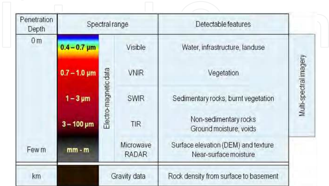
Fig. 3. Spectral overview of electro-magnetic satellite imagery
