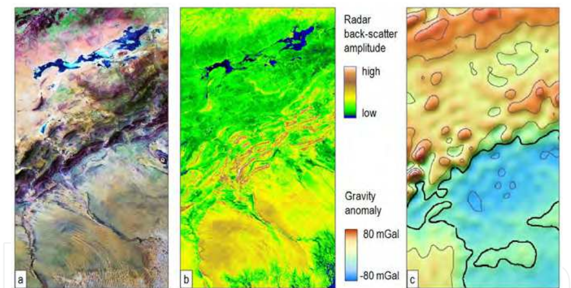
Fig. 5. Examples for optical and radar satellite imagery: a – optical data [Landsat 742 RGB] for comparison, b – radar scatter intensity [Radarsat-1], c – gravity anomaly derived from radar
