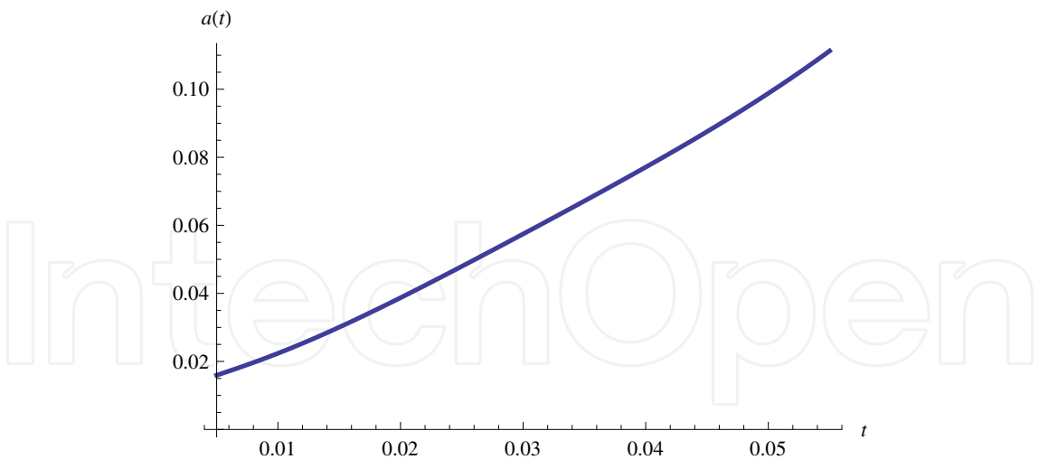
Fig. 7. The time evolution of the radius a(t) of the universe. As it is expected the radius increases monotonically during the expansion. Time is in arbitrary units.
