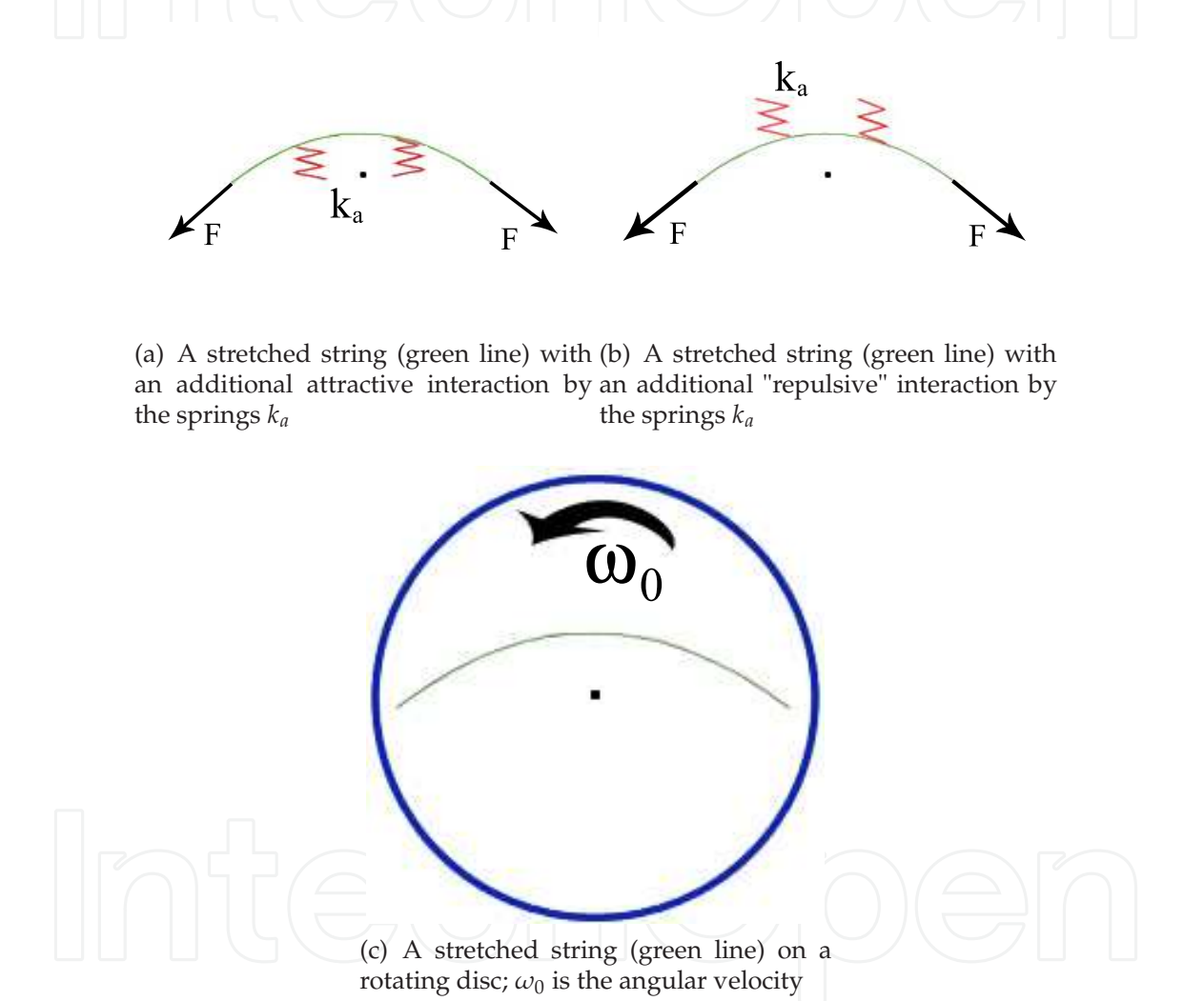
Fig. 2. The three physical situations of the stretched string; the acting force is F for each cases. The equations of motion due to the attractive or "repulsive" interactions pertain to the different figures: Equation (15) for Fig. (a); Equation (16) for Fig. (b); Equation (18) for Fig. (c).
