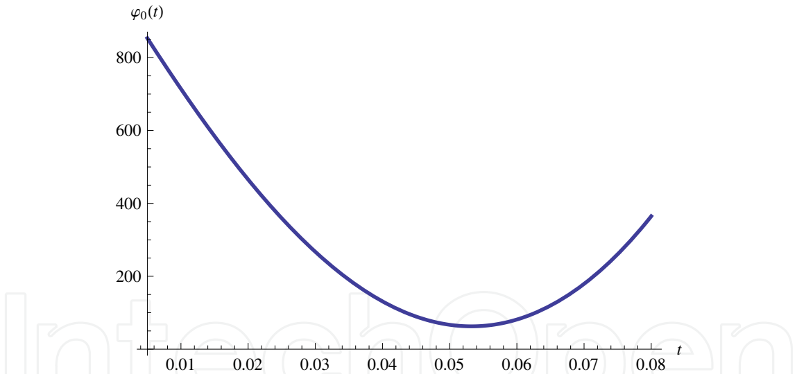
Fig. 4. The time evolution of the thermal field \phi_0(t) . The field decays in the first period and reaches its minimal value. It begins to increase monotonically when the inflaton field \phi_0(t) starts to oscillate. Time is in arbitrary units.
