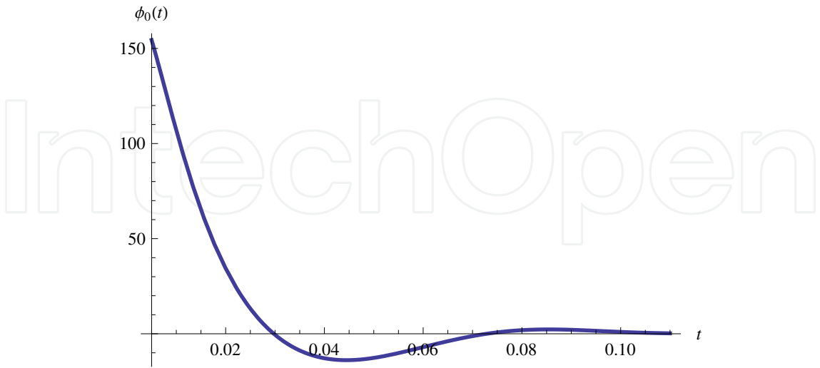
Fig. 3. The time evolution of the inflaton field \phi_0(t) is shown. The short decreasing (deacying) period is followed by a rather long damped oscillating process. Time is in arbitrary units.
