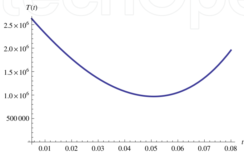
Fig. 5. The time evolution of the temperature field T(t) . The temperature follows the change of the thermal field \varphi_0 . It decreases in the first period of the expansion while its reaches a minimal value. The, due to the pumping of the inflaton field \phi_0 into the thermal field \varphi_0 , the temperature starts increasing. This growing temperature period can be identified as the reheating process in Linde’s cosmology model. Time is in arbitrary units.
