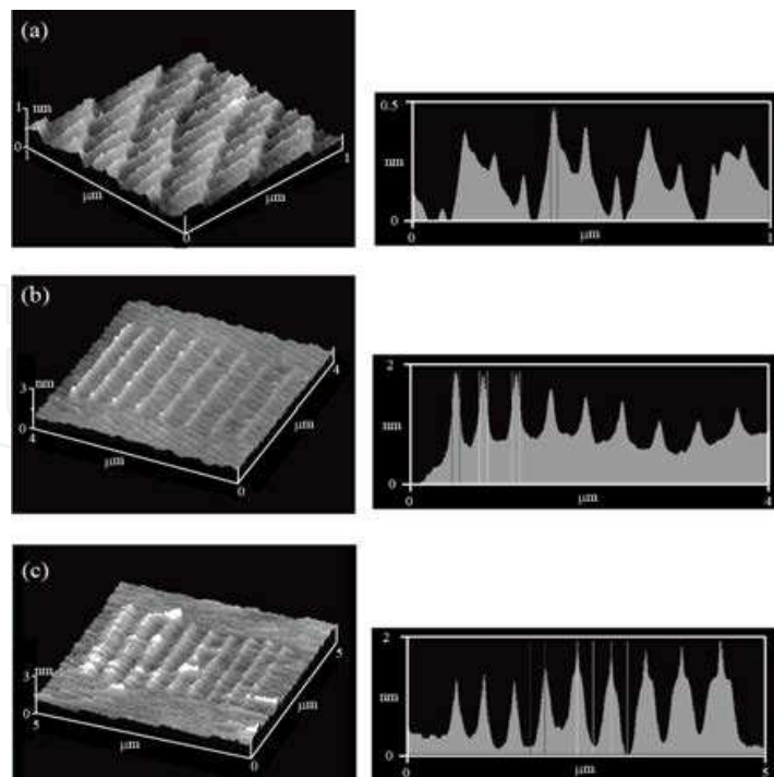
Fig. 4. The topographic images of SiOx line structure fabricated on the 1-decane monolayer and profiles for each topographic image by using various tip: (a) diamond coated Si tip, (b) Si tip and (c) Au coated Si tip. [SH. Lee, N. Saito, O. Takai, Highly reproducible technique for three-dimensional nanostructure fabrication via anodization scanning probe lithography, Appl. Surf. Sci. , 255, 7302-7306 (2009). Copyright@ELSEVIER (2009)]
