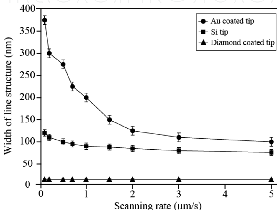
Fig. 5. The change of the line width with increasing scanning rate [SH. Lee, N. Saito, O. Takai, Highly reproducible technique for three-dimensional nanostructure fabrication via anodization scanning probe lithography, Appl. Surf. Sci. , 255, 7302-7306 (2009). Copyright@ELSEVIER (2009)]
