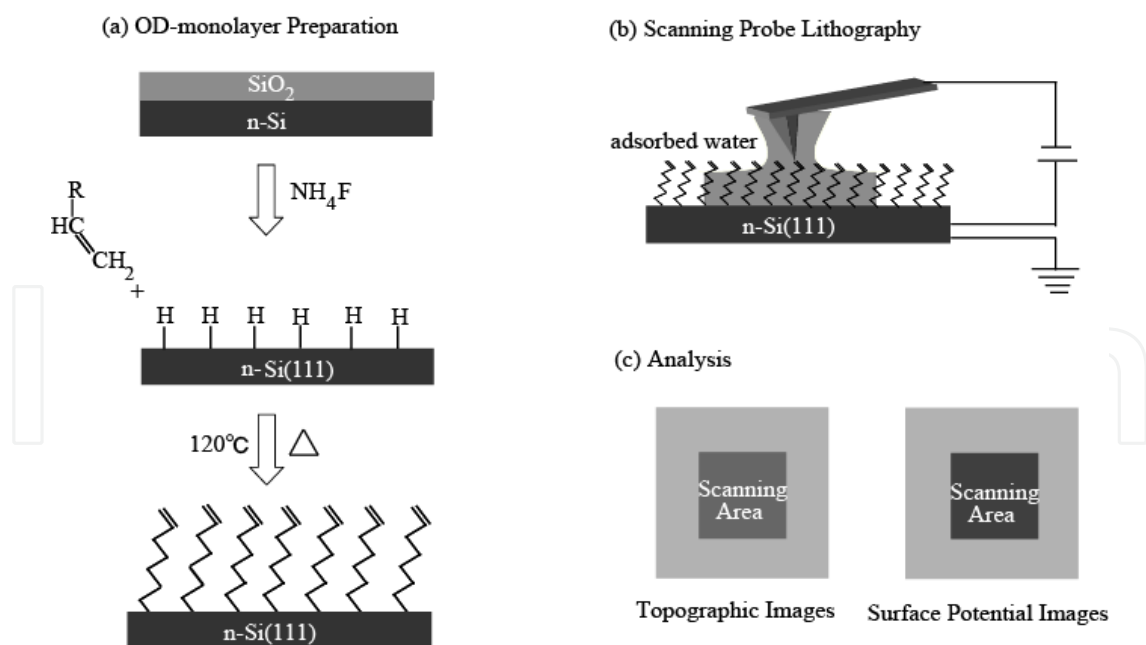
Fig. 16. Schematic illustrations of the experimental process: (a) preparation of the OD-monolayer, (b) electrochemical scanning probe lithography and (c) chemical conversion analysis. [SH. Lee, T. Ishizaki, N. Saito, O. Takai, Electrochemical Soft Lithography of an 1,7-octadiene Monolayer Covalently Linked to Hydrogen-Terminated Silicon using Scanning Probe Microscope, Surf. Sci. , 601, 4206-4211 (2007). Copyright@ELSEVIER (2007)]
