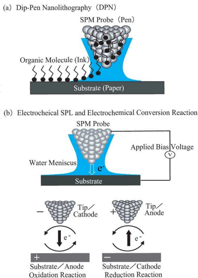
Fig. 2. Schematic illustration of dip-pen nanolithography (DPN) and electrochemical SPL.
