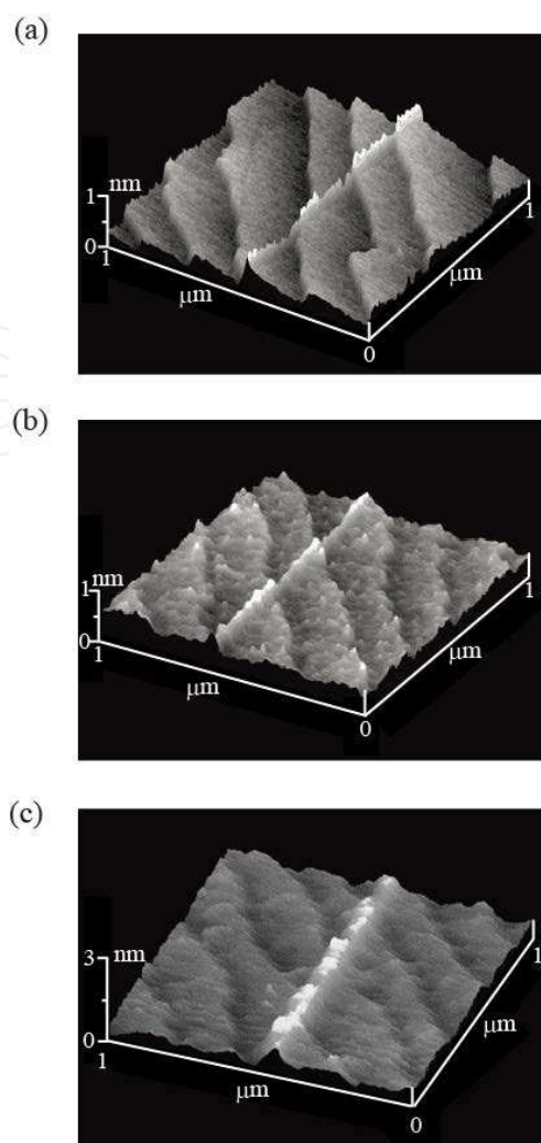
Fig. 6. Topographic images of line structure fabricated by (a) diamond coated Si tip, (b) Si tip and (c) Au coated Si tip, respectively. The applied bias voltage and scanning rate are 7 V and 1 \mu\text{m/s} , respectively. [SH. Lee, N. Saito, O. Takai, Highly reproducible technique for three-dimensional nanostructure fabrication via anodization scanning probe lithography, Appl. Surf. Sci., 255, 7302-7306 (2009). Copyright@ELSEVIER (2009)]
