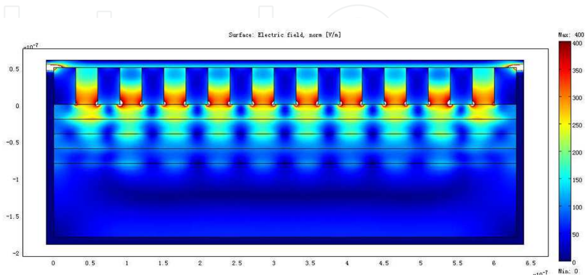
Fig. 2. Electric field distribution of dual-layered heterostructure for CD=30nm.
