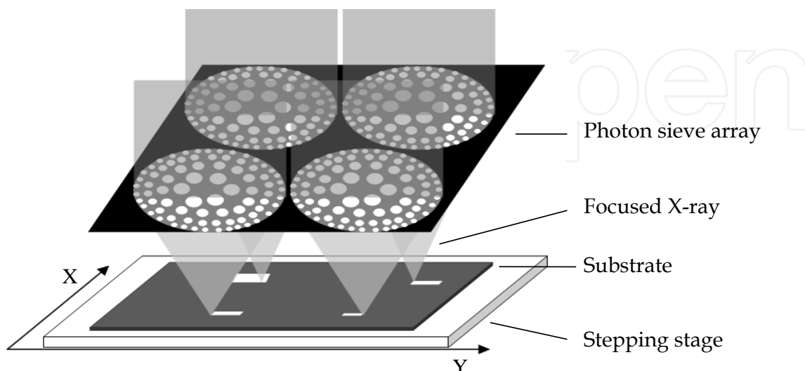
Fig. 1. Schematic of PSAL. An array of photon sieves focuses incident X-ray into a matrix of spots on the substrate coated photoresist. Patterns of arbitrary geometry are recorded while the stepping stage is driven.
