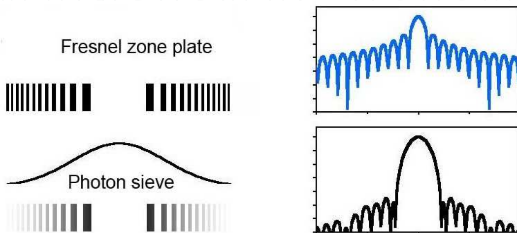
Fig. 3. Schematic of photon sieve suppressing side lobes.
