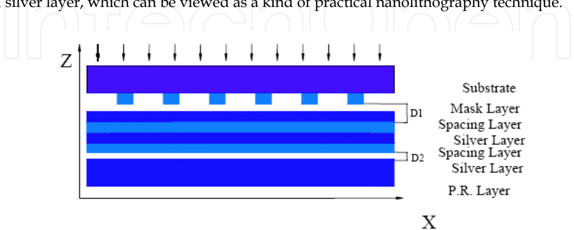
Fig. 10. Sketch of Nanolithography Model.
