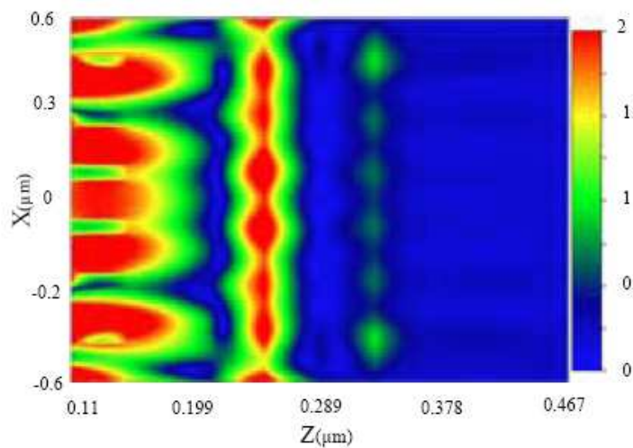
Fig. 15. The distribution of electromagnetic field in the model (Both X and Z is in unit of \mu\text{m} . Photoresist layer lies between Z=0.37\mu\text{m} and Z=0.47\mu\text{m} ).
