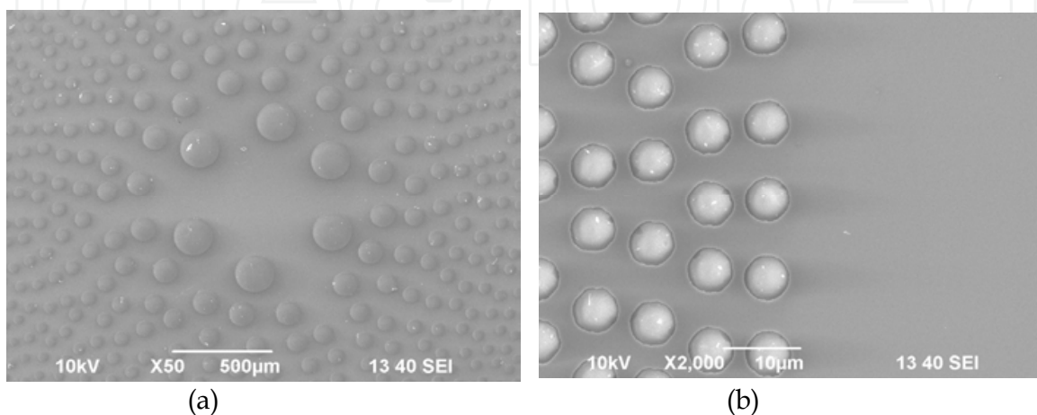
Fig. 8. Scanning electron microscope images of an amplitude-photon sieve. (a) Central portion, (b) the outermost portion.
