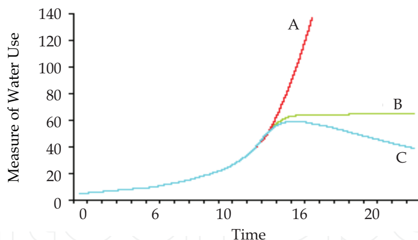
Fig. 1. Scenarios of future water use. (Gliek, 2003)
