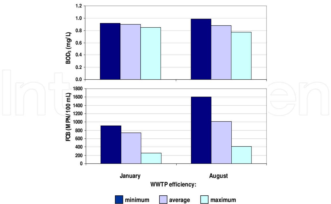
Fig. 18. Concentrations results for BOD 5 and FCB under scenarios 14 to 17 at Ponte Nova Barcelos in river Cávado
