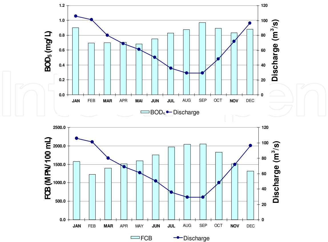
Fig. 17. Concentrations results for BOD 5 and FCB for scenarios 2 to 13 at Ponte Nova de Barcelos in river Cávado
