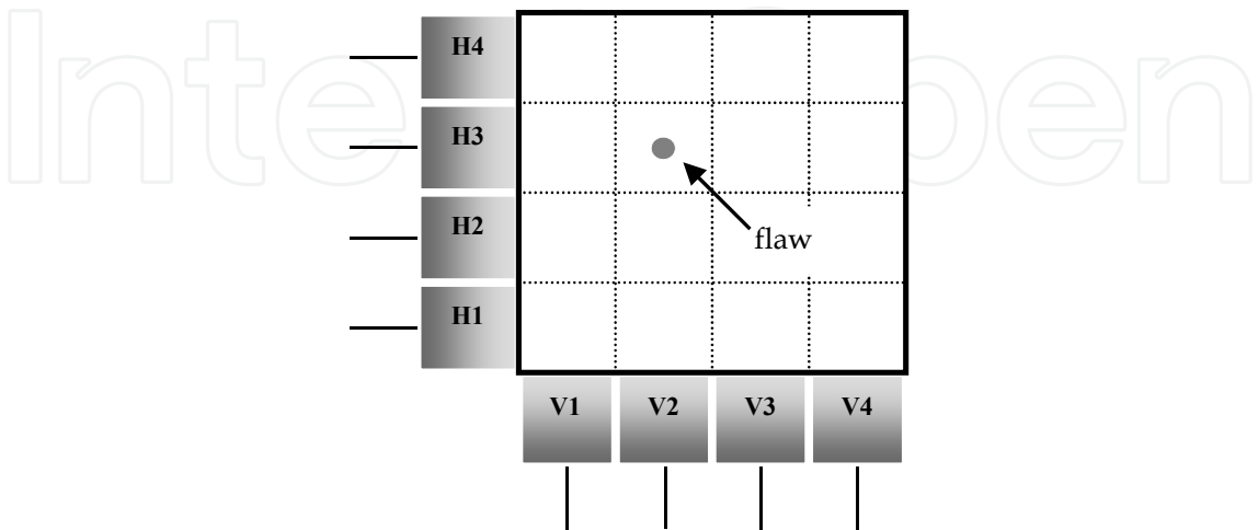
Fig. 4. Geometry of the inspection case planned to evaluate the different combination methods: detection of a single-flaw in a 2D arrangement with 16 elemental-cells.
