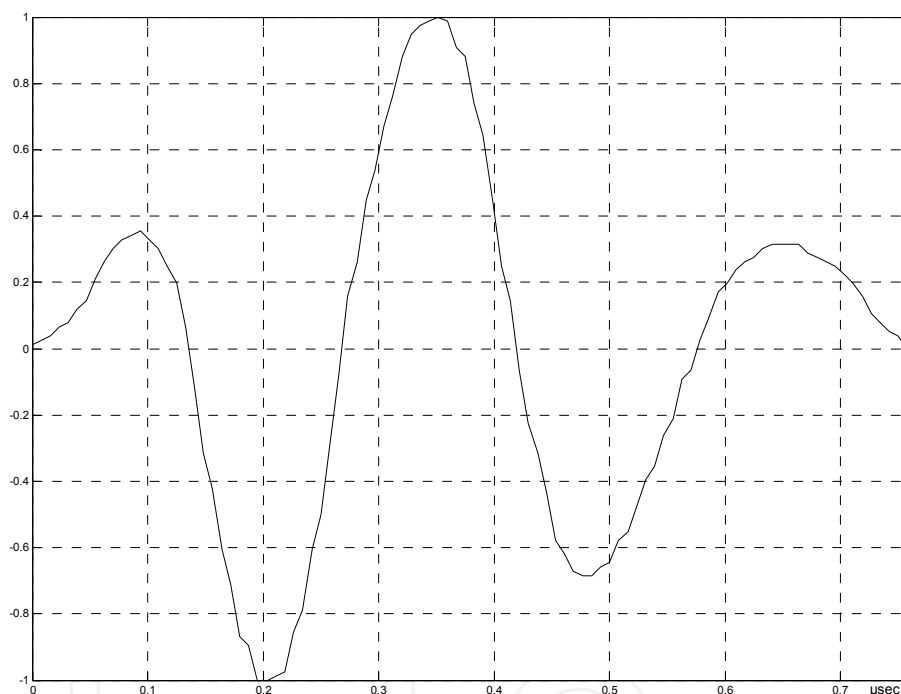
Fig. 5. Ultrasonic echo utilised in type-I experiments.
