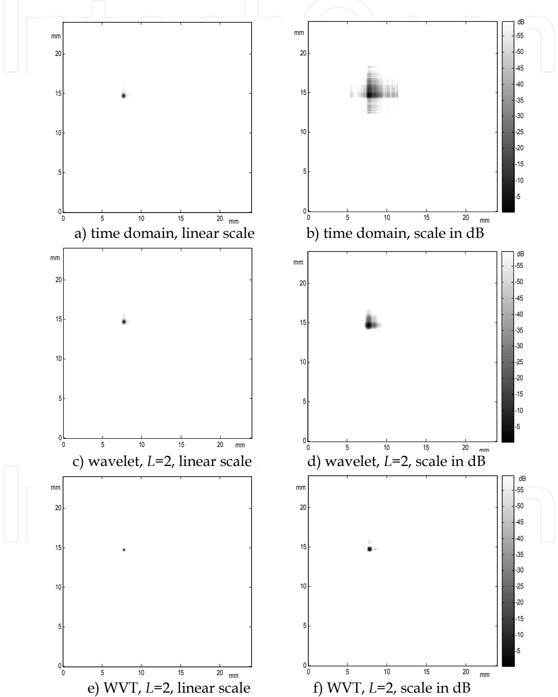
Fig. 9. Different 2D representations after combination of real traces in experiments type-II, with linear scale (a, c, e) and logarithmic scale (b, d, f).
